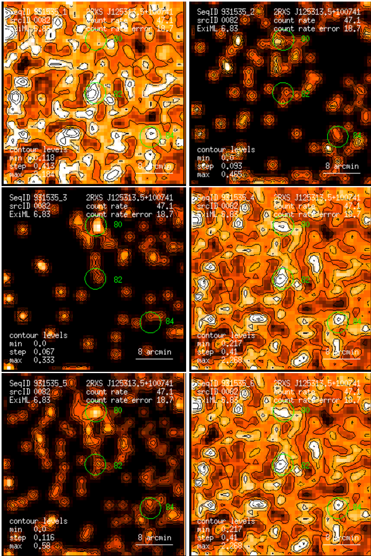
Figure 82: RASS 931535: detection 0082: band rate images, Gaussian filter: (1) PSPC channels 11 – 41, (2) 52 – 90, (3) 91 – 201, (4) 11 – 235, (5) 52 – 201, (6) 11 – 201. Broad band rates in counts/ks. Band rate contour levels in counts/ks/arcmin 2 .
