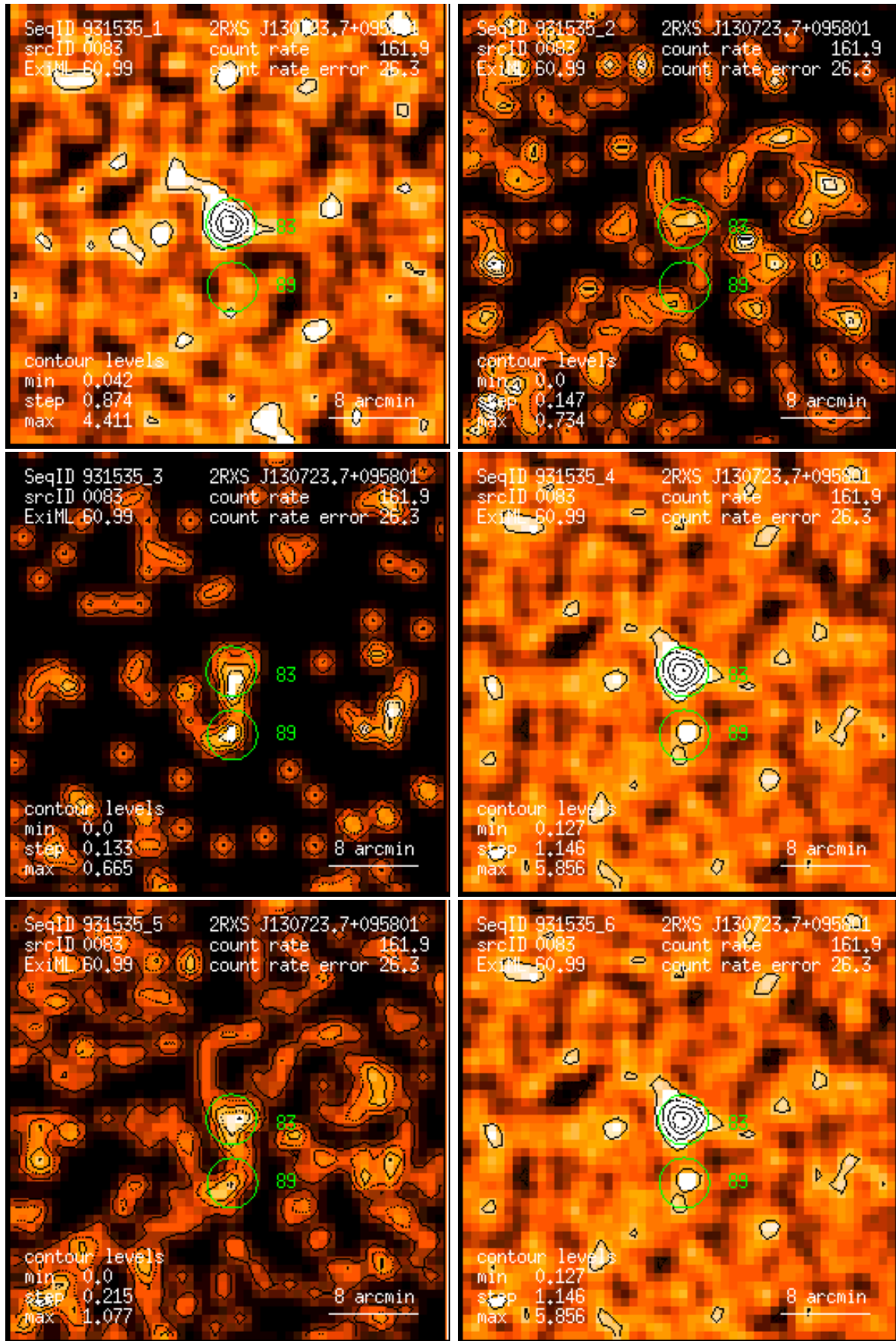
Figure 83: RASS 931535: detection 0083: band rate images, Gaussian filter: (1) PSPC channels 11 – 41, (2) 52 – 90, (3) 91 – 201, (4) 11 – 235, (5) 52 – 201, (6) 11 – 201. Broad band rates in counts/ks. Band rate contour levels in counts/ks/arcmin 2 .
