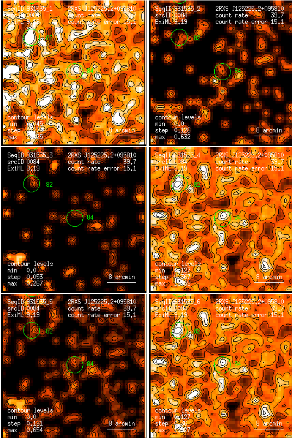
Figure 84: RASS 931535: detection 0084: band rate images, Gaussian filter: (1) PSPC channels 11 – 41, (2) 52 – 90, (3) 91 – 201, (4) 11 – 235, (5) 52 – 201, (6) 11 – 201. Broad band rates in counts/ks. Band rate contour levels in counts/ks/arcmin 2 .
