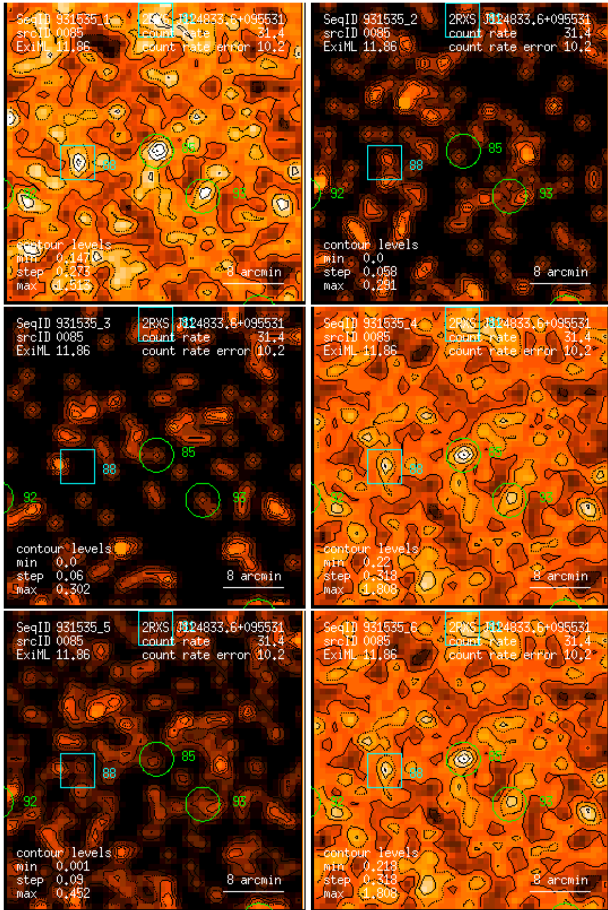
Figure 85: RASS 931535: detection 0085: band rate images, Gaussian filter: (1) PSPC channels 11 – 41, (2) 52 – 90, (3) 91 – 201, (4) 11 – 235, (5) 52 – 201, (6) 11 – 201. Broad band rates in counts/ks. Band rate contour levels in counts/ks/arcmin 2 .
