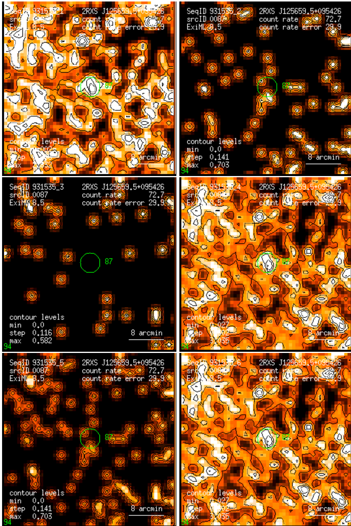
Figure 87: RASS 931535: detection 0087: band rate images, Gaussian filter: (1) PSPC channels 11 – 41, (2) 52 – 90, (3) 91 – 201, (4) 11 – 235, (5) 52 – 201, (6) 11 – 201. Broad band rates in counts/ks. Band rate contour levels in counts/ks/arcmin 2 .
