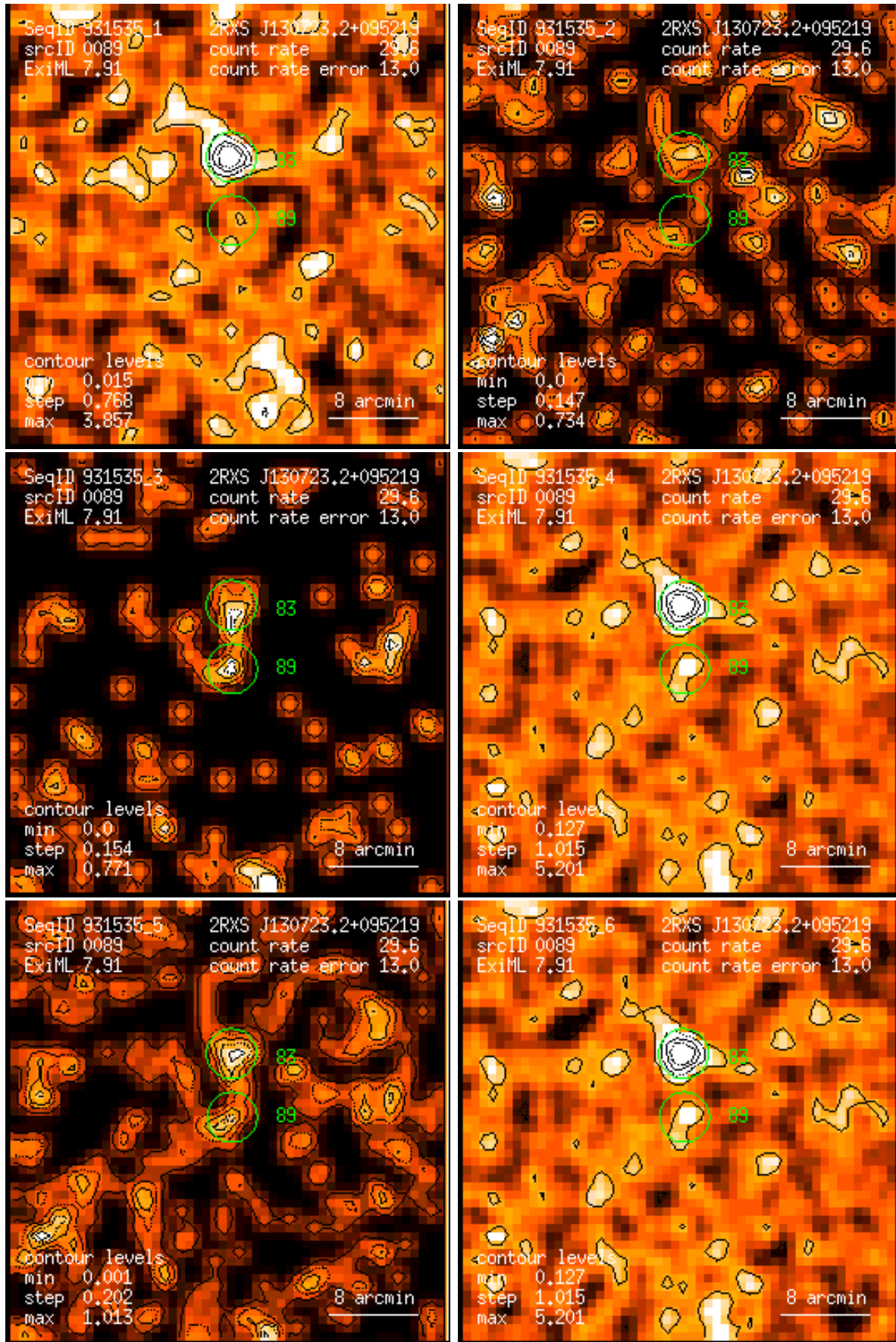
Figure 89: RASS 931535: detection 0089: band rate images, Gaussian filter: (1) PSPC channels 11 – 41, (2) 52 – 90, (3) 91 – 201, (4) 11 – 235, (5) 52 – 201, (6) 11 – 201. Broad band rates in counts/ks. Band rate contour levels in counts/ks/arcmin 2 .
