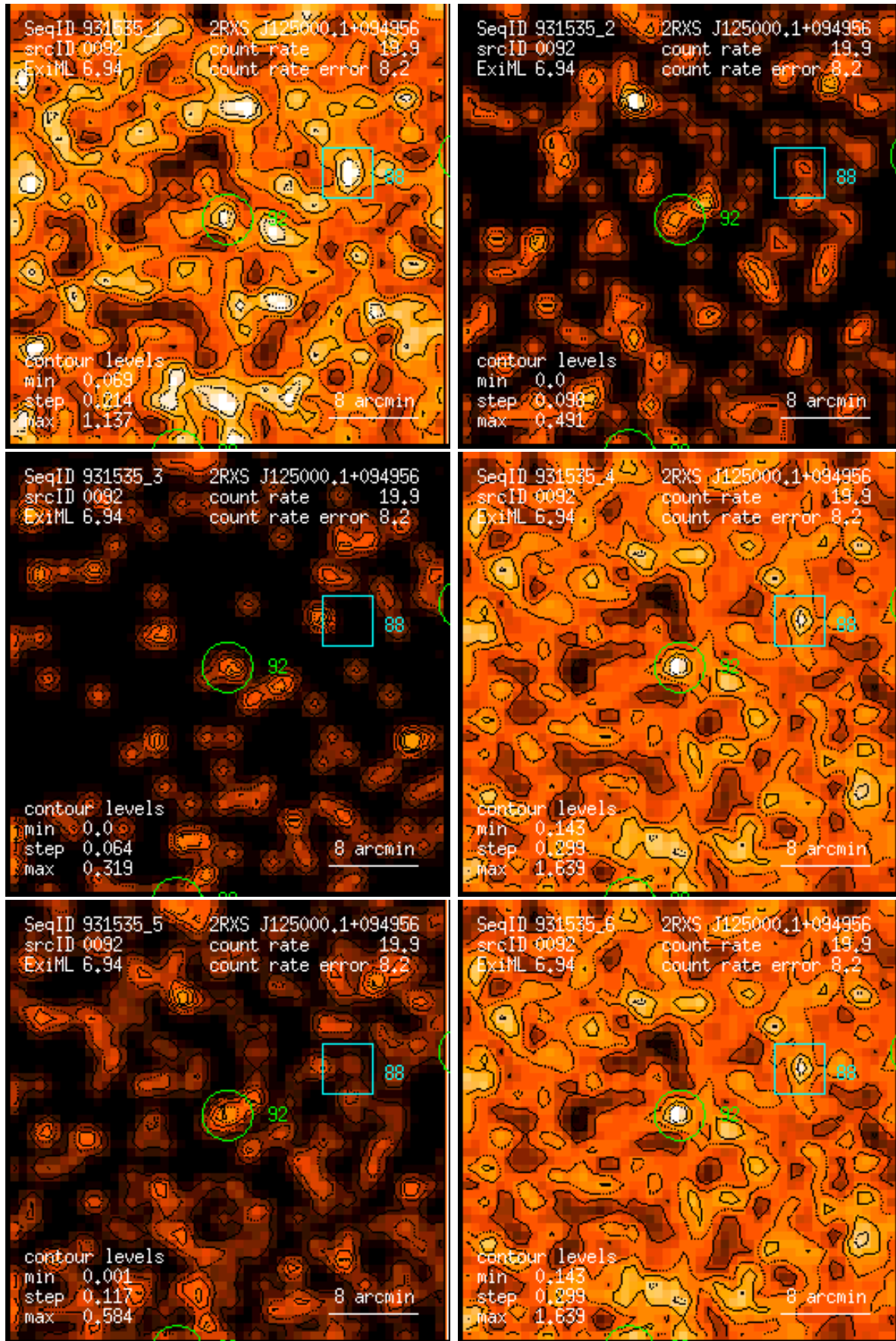
Figure 92: RASS 931535: detection 0092: band rate images, Gaussian filter: (1) PSPC channels 11 – 41, (2) 52 – 90, (3) 91 – 201, (4) 11 – 235, (5) 52 – 201, (6) 11 – 201. Broad band rates in counts/ks. Band rate contour levels in counts/ks/arcmin 2 .
