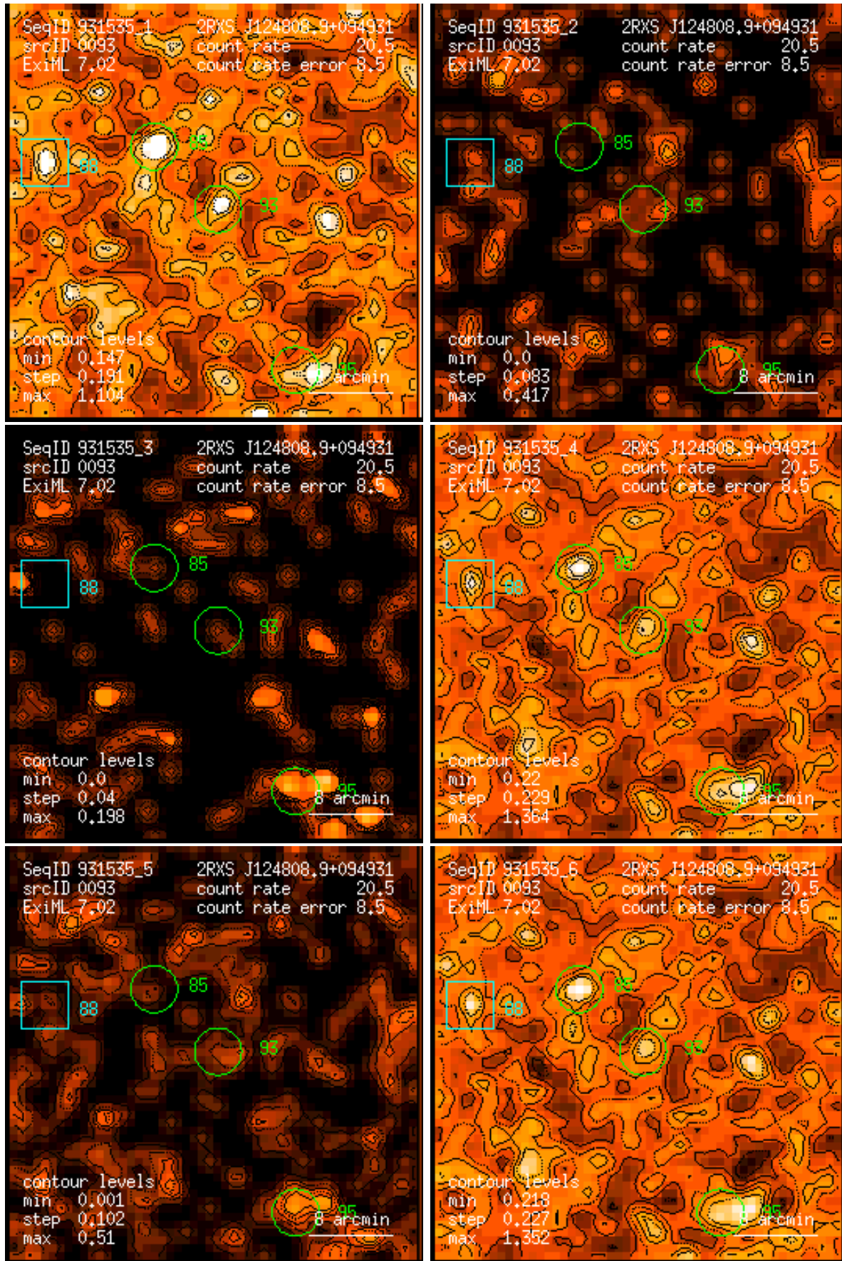
Figure 93: RASS 931535: detection 0093: band rate images, Gaussian filter: (1) PSPC channels 11 – 41, (2) 52 – 90, (3) 91 – 201, (4) 11 – 235, (5) 52 – 201, (6) 11 – 201. Broad band rates in counts/ks. Band rate contour levels in counts/ks/arcmin 2 .
