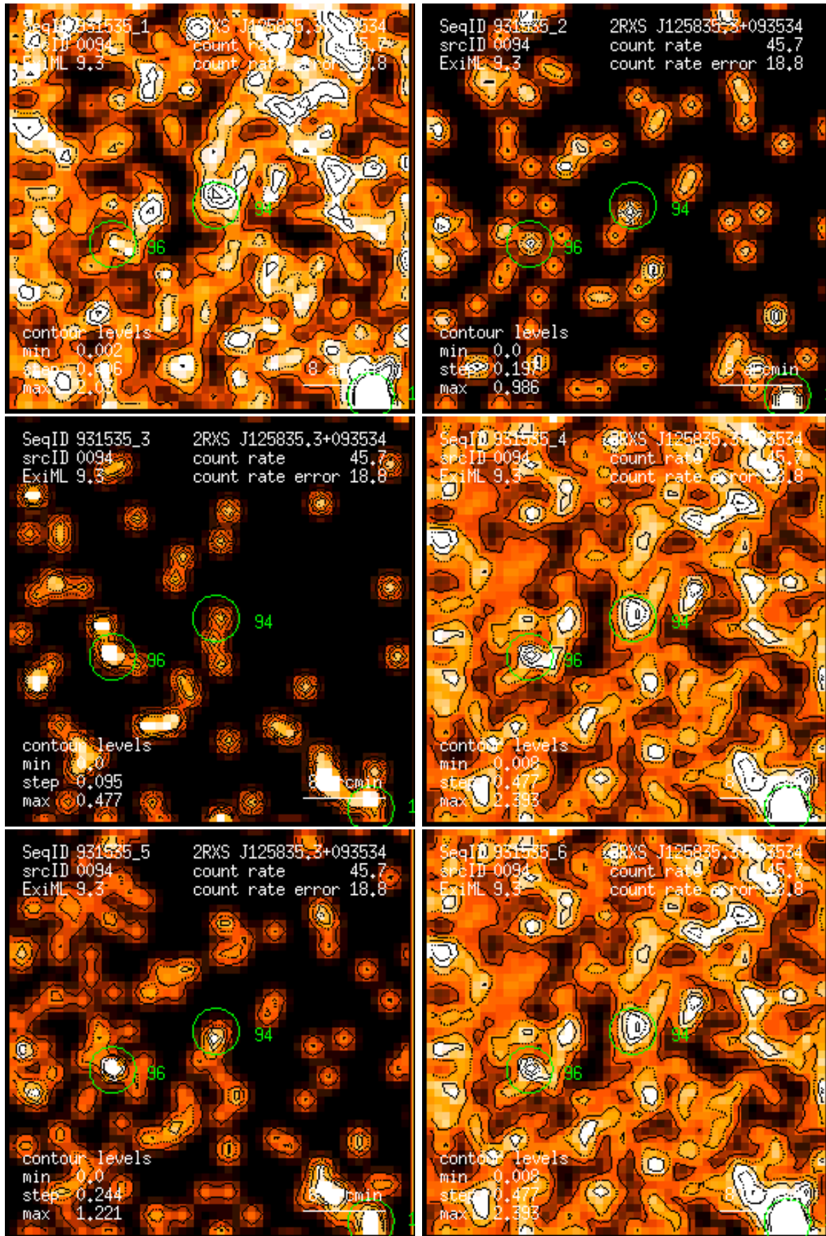
Figure 94: RASS 931535: detection 0094: band rate images, Gaussian filter: (1) PSPC channels 11 – 41, (2) 52 – 90, (3) 91 – 201, (4) 11 – 235, (5) 52 – 201, (6) 11 – 201. Broad band rates in counts/ks. Band rate contour levels in counts/ks/arcmin 2 .
