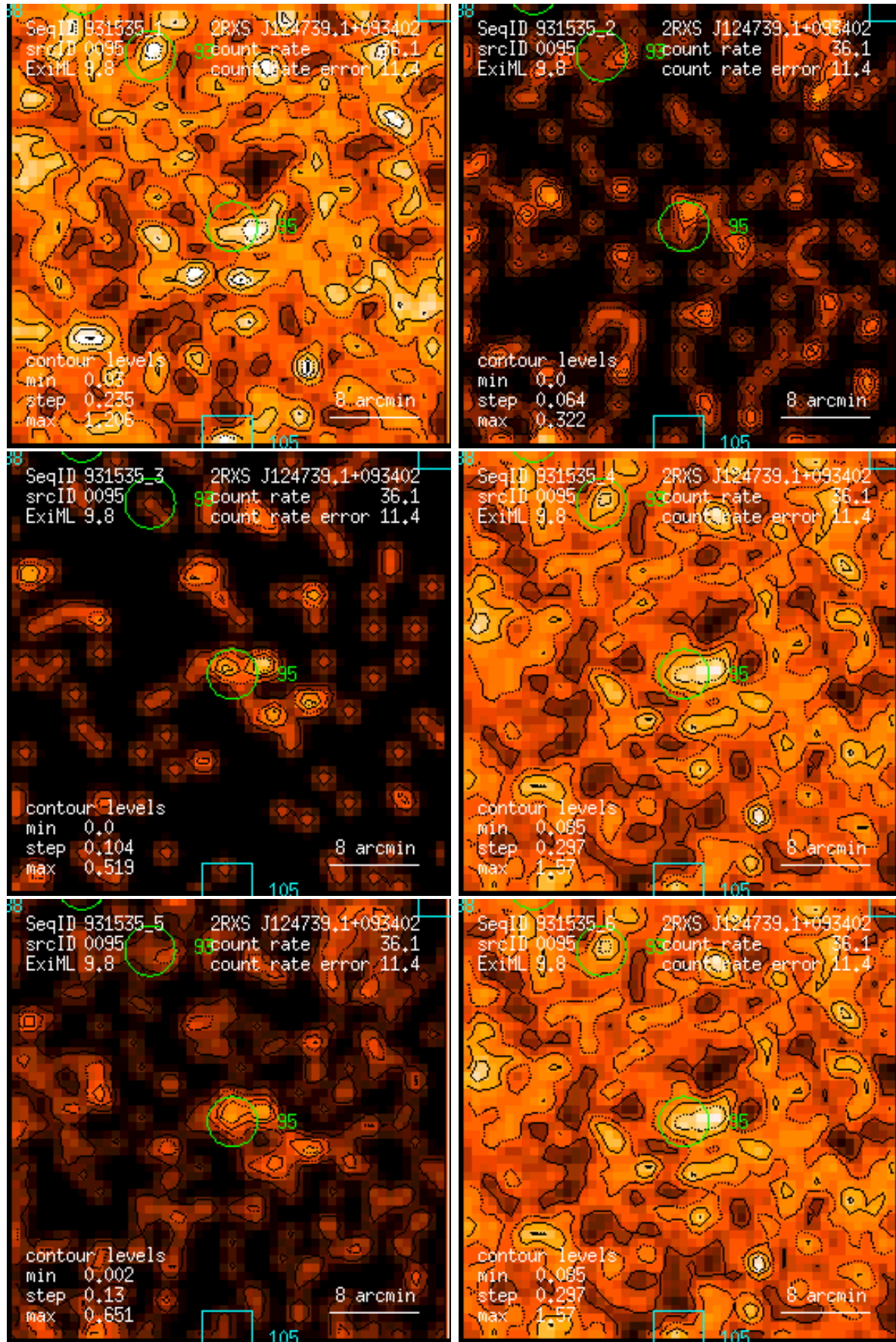
Figure 95: RASS 931535: detection 0095: band rate images, Gaussian filter: (1) PSPC channels 11 – 41, (2) 52 – 90, (3) 91 – 201, (4) 11 – 235, (5) 52 – 201, (6) 11 – 201. Broad band rates in counts/ks. Band rate contour levels in counts/ks/arcmin 2 .
