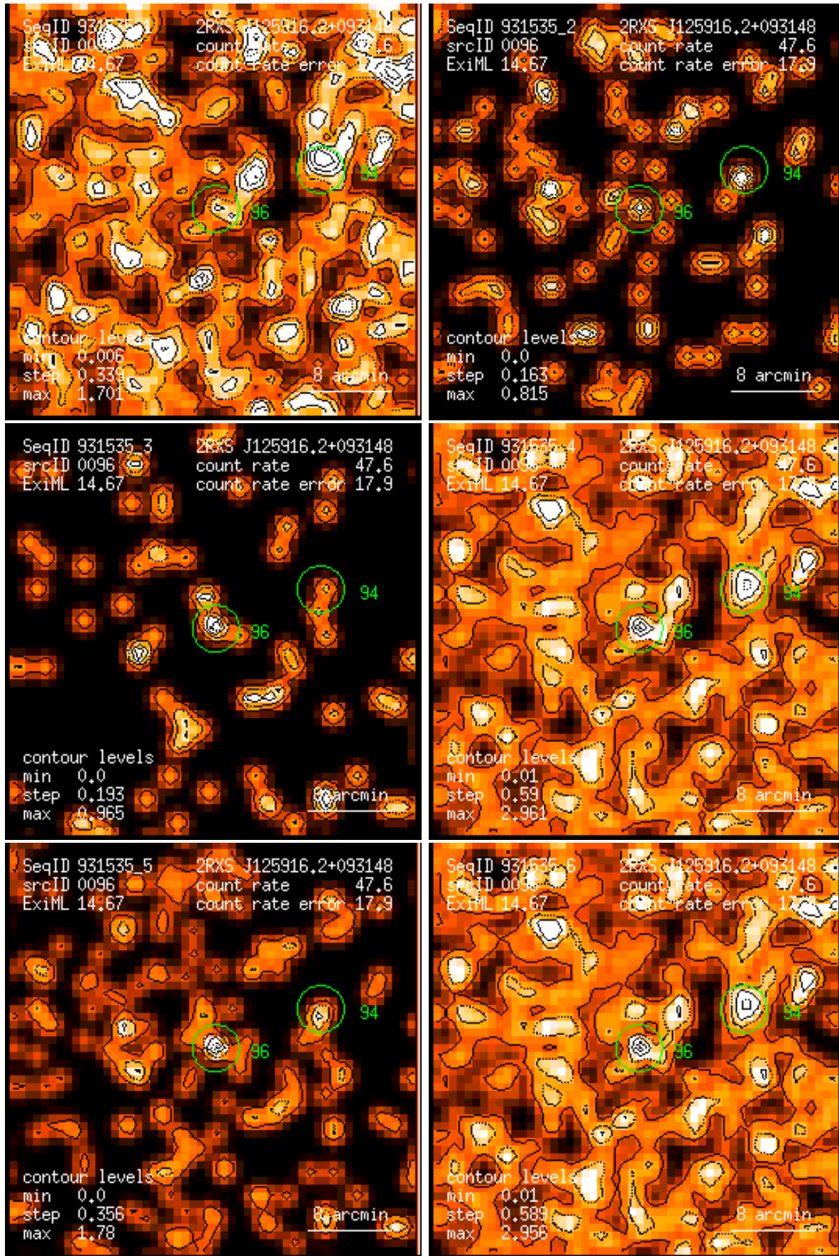
Figure 96: RASS 931535: detection 0096: band rate images, Gaussian filter: (1) PSPC channels 11 – 41, (2) 52 – 90, (3) 91 – 201, (4) 11 – 235, (5) 52 – 201, (6) 11 – 201. Broad band rates in counts/ks. Band rate contour levels in counts/ks/arcmin 2 .
