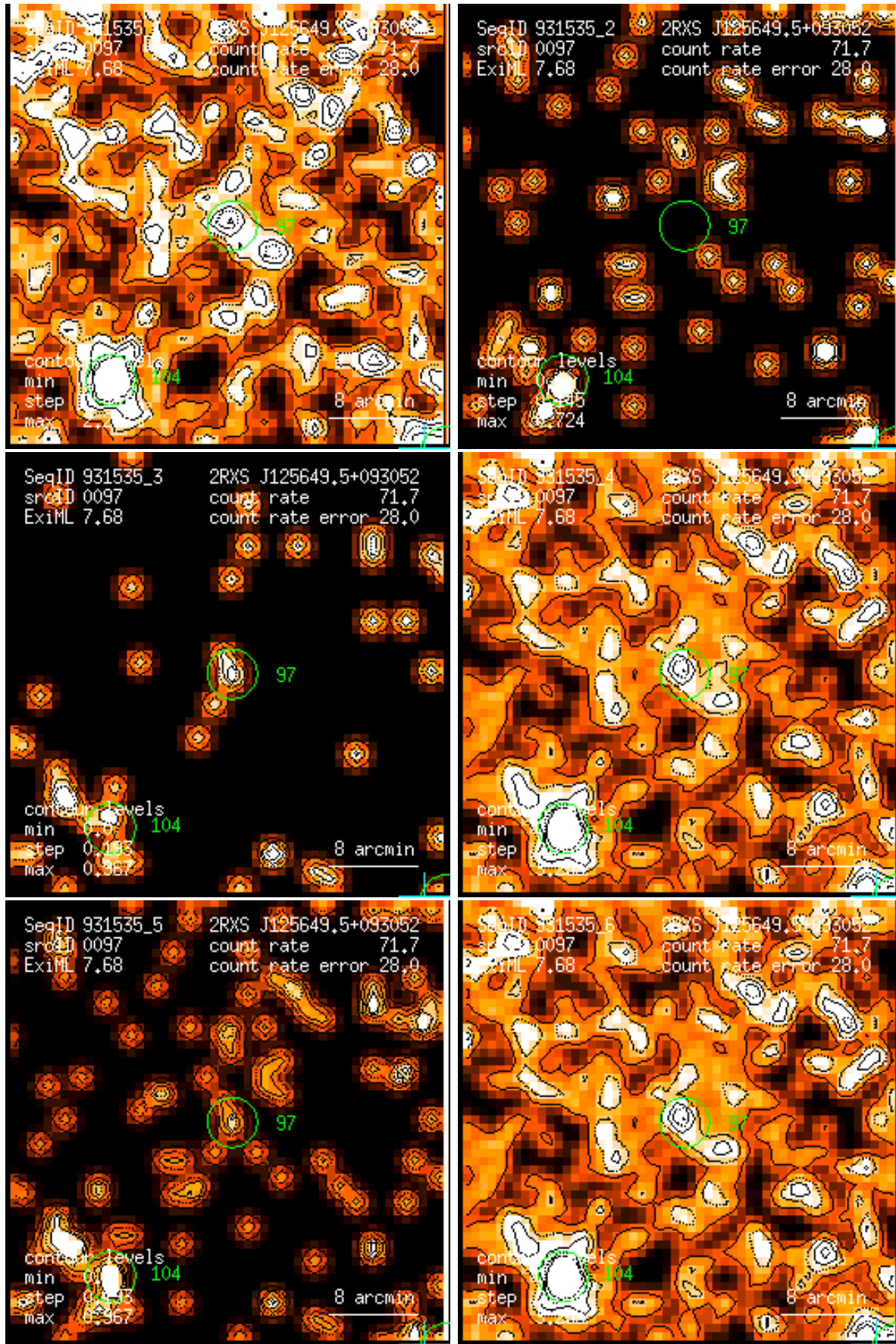
Figure 97: RASS 931535: detection 0097: band rate images, Gaussian filter: (1) PSPC channels 11 – 41, (2) 52 – 90, (3) 91 – 201, (4) 11 – 235, (5) 52 – 201, (6) 11 – 201. Broad band rates in counts/ks. Band rate contour levels in counts/ks/arcmin 2 .
