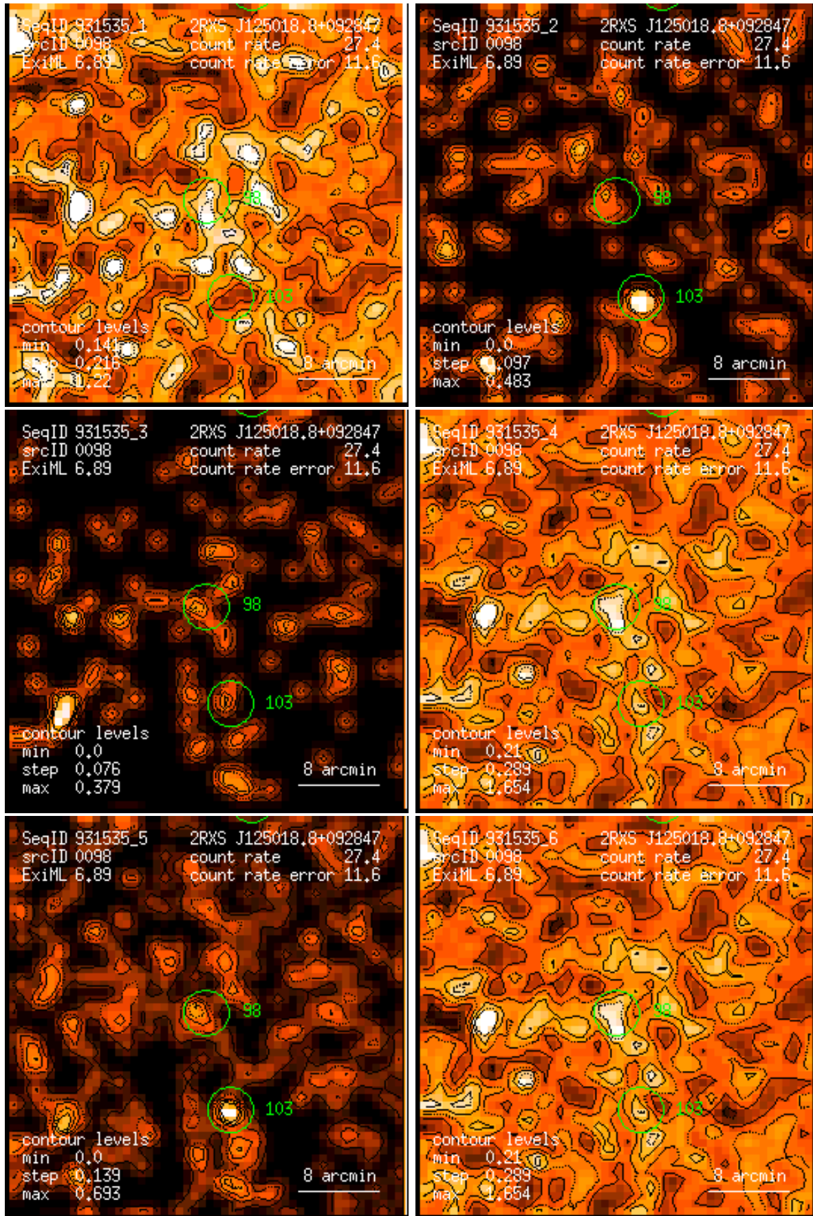
Figure 98: RASS 931535: detection 0098: band rate images, Gaussian filter: (1) PSPC channels 11 – 41, (2) 52 – 90, (3) 91 – 201, (4) 11 – 235, (5) 52 – 201, (6) 11 – 201. Broad band rates in counts/ks. Band rate contour levels in counts/ks/arcmin 2 .
