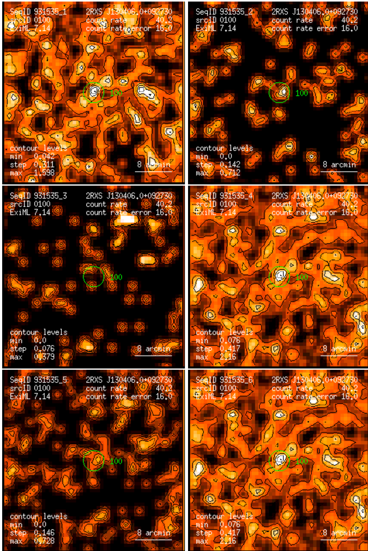
Figure 100: RASS 931535: detection 0100: band rate images, Gaussian filter: (1) PSPC channels 11 – 41, (2) 52 – 90, (3) 91 – 201, (4) 11 – 235, (5) 52 – 201, (6) 11 – 201. Broad band rates in counts/ks. Band rate contour levels in counts/ks/arcmin 2 .
