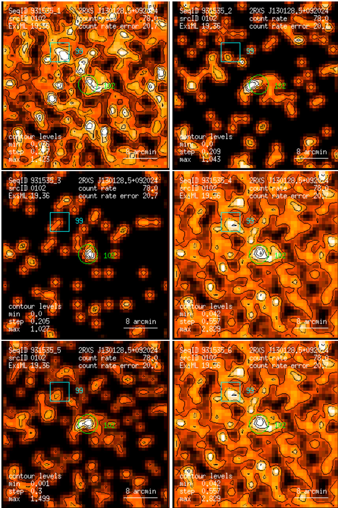
Figure 102: RASS 931535: detection 0102: band rate images, Gaussian filter: (1) PSPC channels 11 – 41, (2) 52 – 90, (3) 91 – 201, (4) 11 – 235, (5) 52 – 201, (6) 11 – 201. Broad band rates in counts/ks. Band rate contour levels in counts/ks/arcmin 2 .
