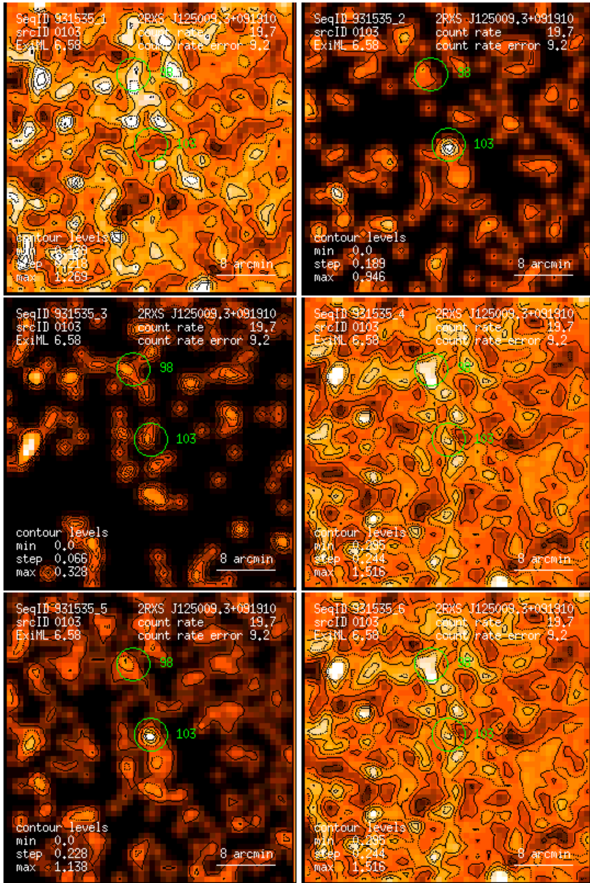
Figure 103: RASS 931535: detection 0103: band rate images, Gaussian filter: (1) PSPC channels 11 – 41, (2) 52 – 90, (3) 91 – 201, (4) 11 – 235, (5) 52 – 201, (6) 11 – 201. Broad band rates in counts/ks. Band rate contour levels in counts/ks/arcmin 2 .
