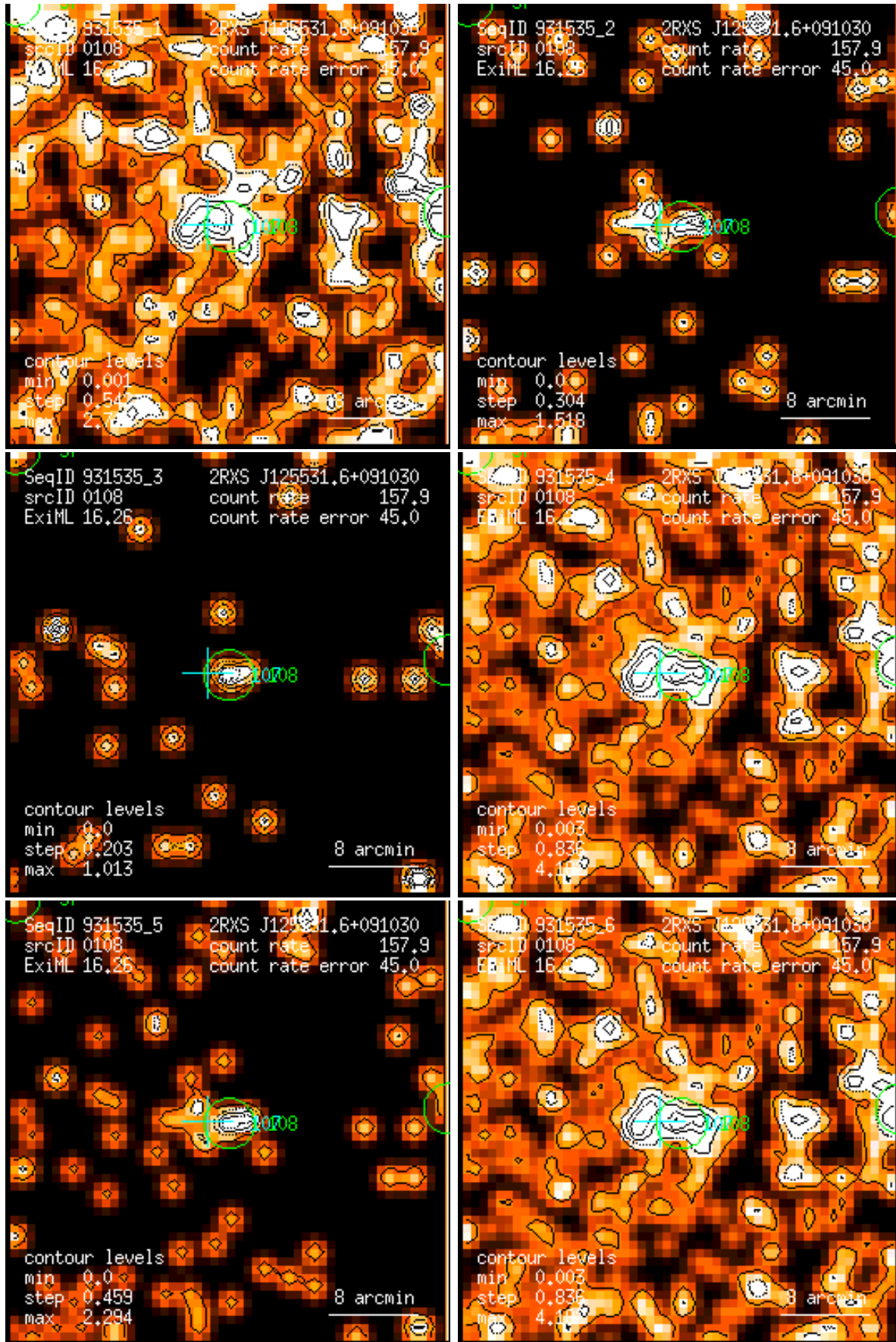
Figure 108: RASS 931535: detection 0108: band rate images, Gaussian filter: (1) PSPC channels 11 – 41, (2) 52 – 90, (3) 91 – 201, (4) 11 – 235, (5) 52 – 201, (6) 11 – 201. Broad band rates in counts/ks. Band rate contour levels in counts/ks/arcmin 2 .
