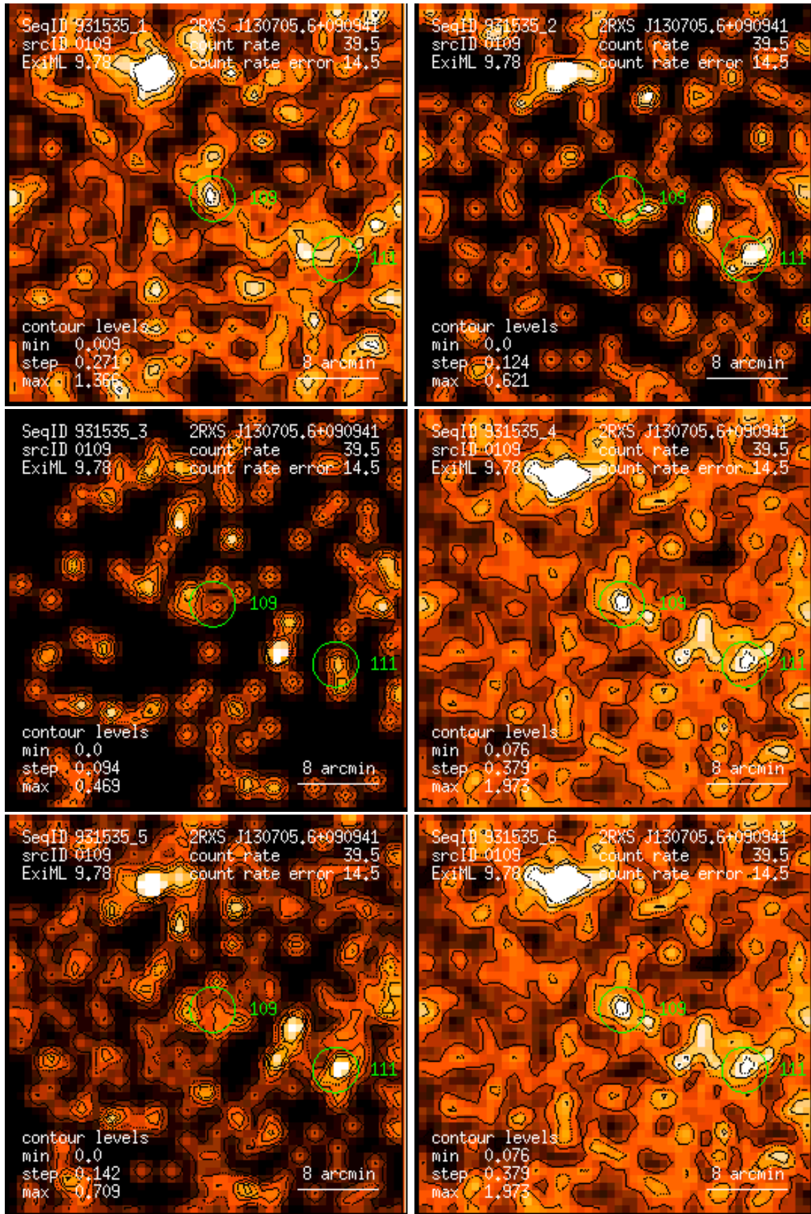
Figure 109: RASS 931535: detection 0109: band rate images, Gaussian filter: (1) PSPC channels 11 – 41, (2) 52 – 90, (3) 91 – 201, (4) 11 – 235, (5) 52 – 201, (6) 11 – 201. Broad band rates in counts/ks. Band rate contour levels in counts/ks/arcmin 2 .
