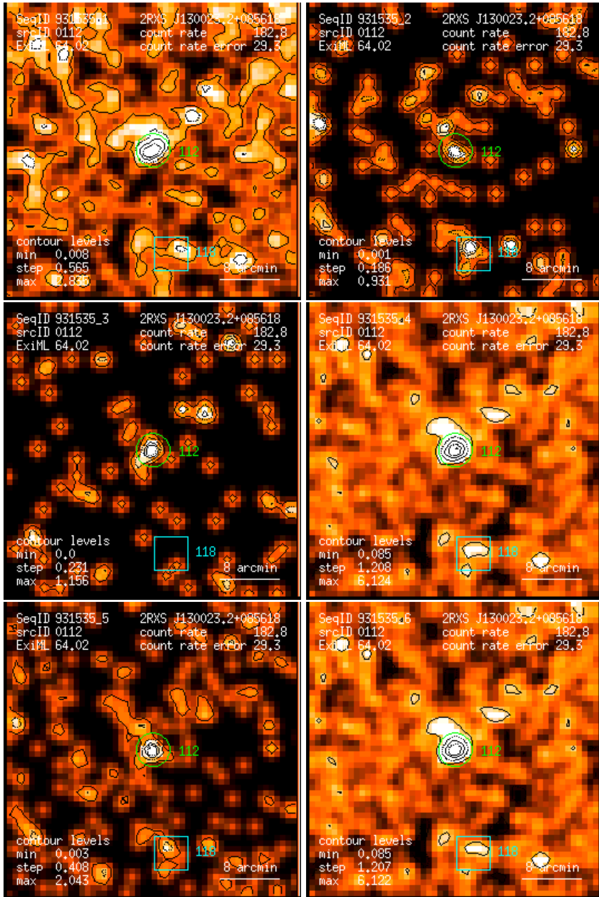
Figure 112: RASS 931535: detection 0112: band rate images, Gaussian filter: (1) PSPC channels 11 – 41, (2) 52 – 90, (3) 91 – 201, (4) 11 – 235, (5) 52 – 201, (6) 11 – 201. Broad band rates in counts/ks. Band rate contour levels in counts/ks/arcmin 2 .
