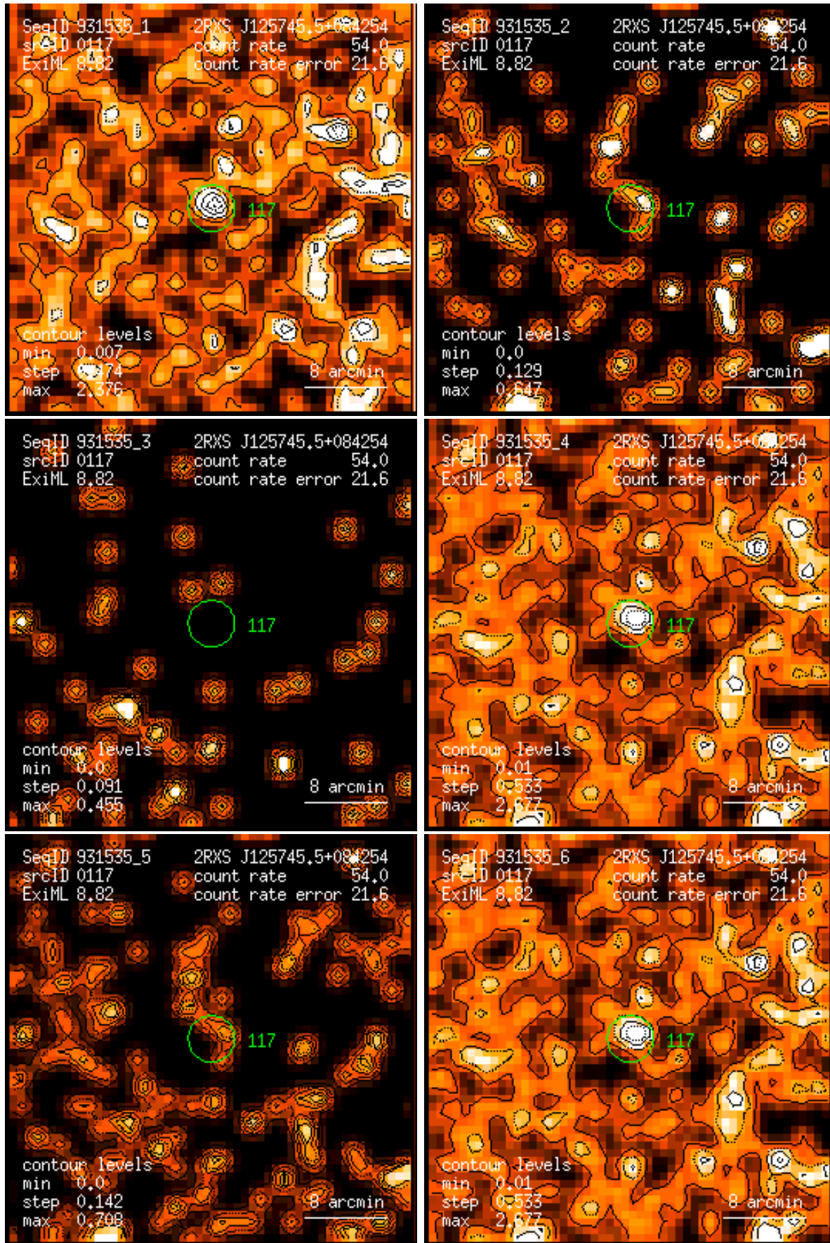
Figure 117: RASS 931535: detection 0117: band rate images, Gaussian filter: (1) PSPC channels 11 – 41, (2) 52 – 90, (3) 91 – 201, (4) 11 – 235, (5) 52 – 201, (6) 11 – 201. Broad band rates in counts/ks. Band rate contour levels in counts/ks/arcmin 2 .
