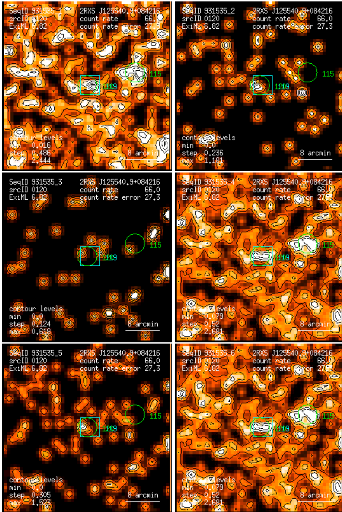
Figure 120: RASS 931535: detection 0120: band rate images, Gaussian filter: (1) PSPC channels 11 – 41, (2) 52 – 90, (3) 91 – 201, (4) 11 – 235, (5) 52 – 201, (6) 11 – 201. Broad band rates in counts/ks. Band rate contour levels in counts/ks/arcmin 2 .
