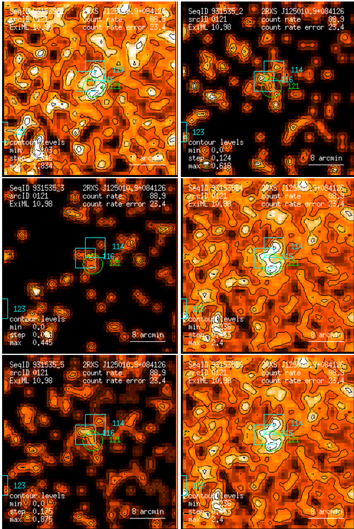
Figure 121: RASS 931535: detection 0121: band rate images, Gaussian filter: (1) PSPC channels 11 – 41, (2) 52 – 90, (3) 91 – 201, (4) 11 – 235, (5) 52 – 201, (6) 11 – 201. Broad band rates in counts/ks. Band rate contour levels in counts/ks/arcmin 2 .
