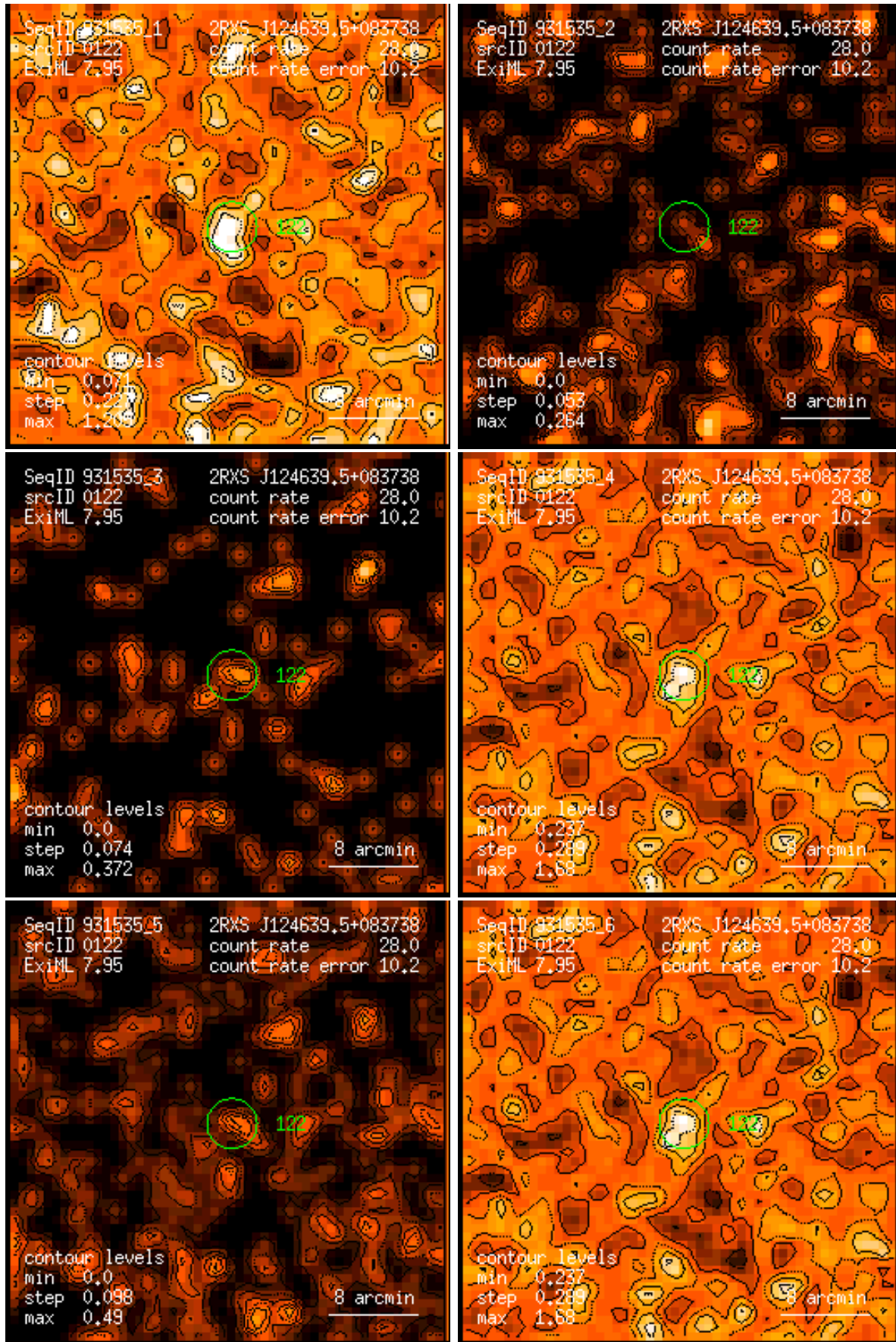
Figure 122: RASS 931535: detection 0122: band rate images, Gaussian filter: (1) PSPC channels 11 – 41, (2) 52 – 90, (3) 91 – 201, (4) 11 – 235, (5) 52 – 201, (6) 11 – 201. Broad band rates in counts/ks. Band rate contour levels in counts/ks/arcmin 2 .
