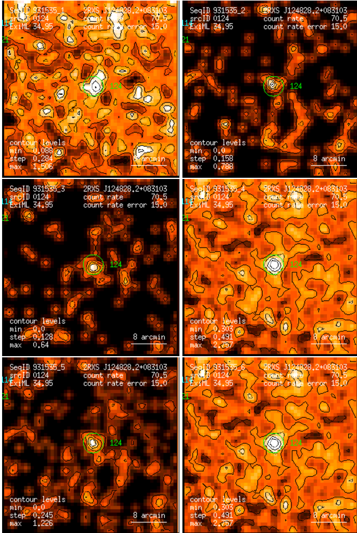
Figure 124: RASS 931535: detection 0124: band rate images, Gaussian filter: (1) PSPC channels 11 – 41, (2) 52 – 90, (3) 91 – 201, (4) 11 – 235, (5) 52 – 201, (6) 11 – 201. Broad band rates in counts/ks. Band rate contour levels in counts/ks/arcmin 2 .
