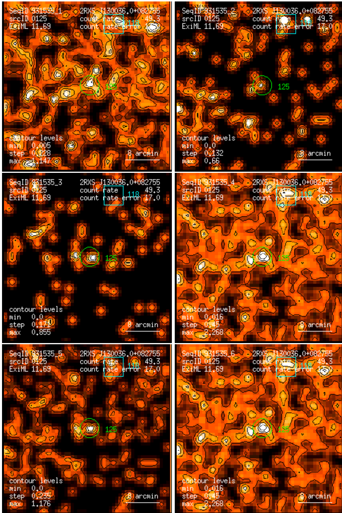
Figure 125: RASS 931535: detection 0125: band rate images, Gaussian filter: (1) PSPC channels 11 – 41, (2) 52 – 90, (3) 91 – 201, (4) 11 – 235, (5) 52 – 201, (6) 11 – 201. Broad band rates in counts/ks. Band rate contour levels in counts/ks/arcmin 2 .
