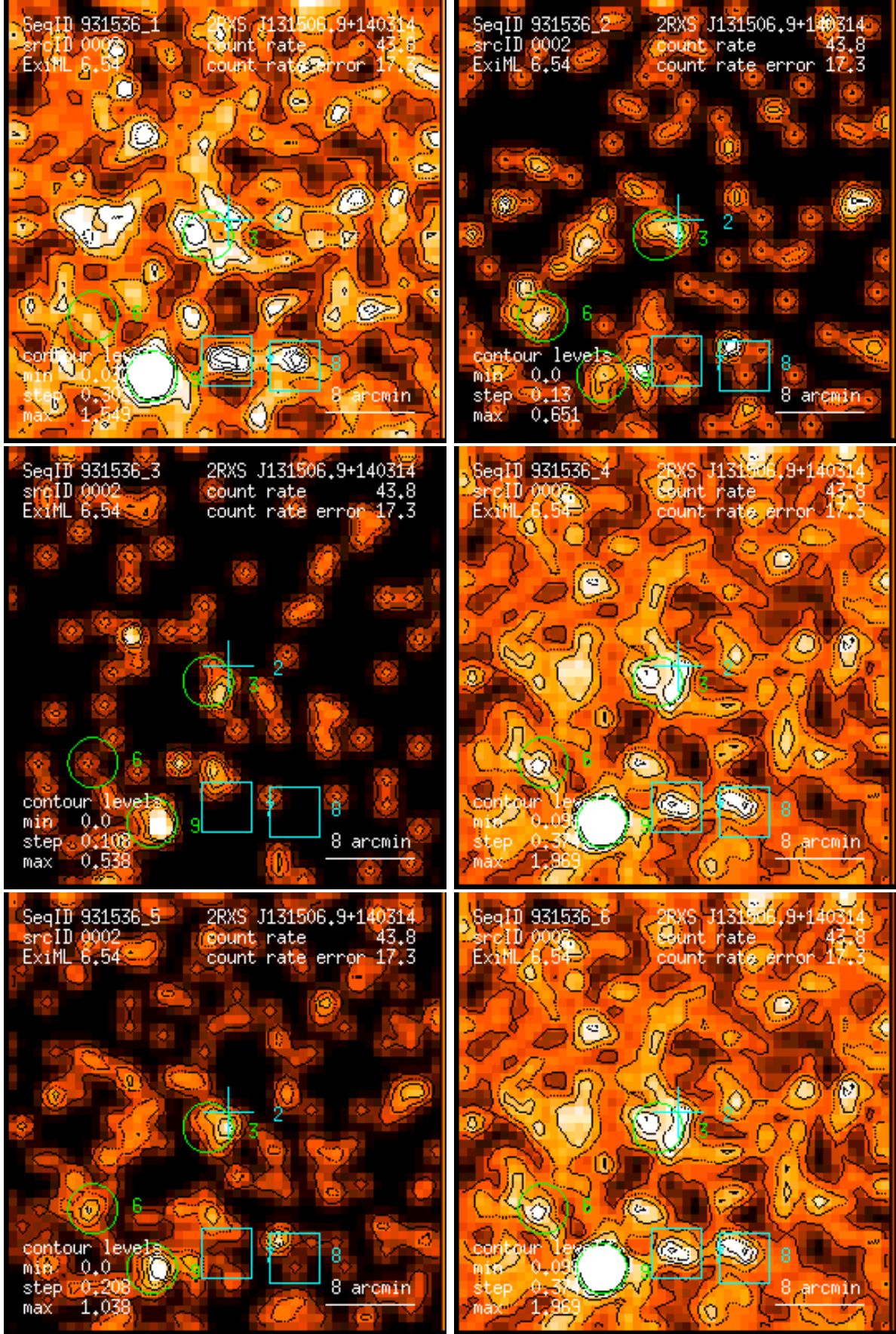
Figure 2: RASS 931536: detection 0002: band rate images, Gaussian filter: (1) PSPC channels 11 – 41, (2) 52 – 90, (3) 91 – 201, (4) 11 – 235, (5) 52 – 201, (6) 11 – 201. Broad band rates in counts/ks. Band rate contour levels in counts/ks/arcmin 2 .
