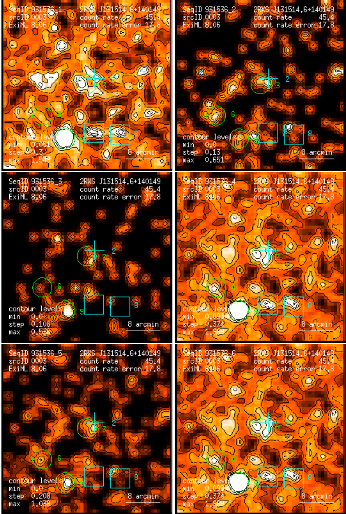
Figure 3: RASS 931536: detection 0003: band rate images, Gaussian filter: (1) PSPC channels 11 – 41, (2) 52 – 90, (3) 91 – 201, (4) 11 – 235, (5) 52 – 201, (6) 11 – 201. Broad band rates in counts/ks. Band rate contour levels in counts/ks/arcmin 2 .
