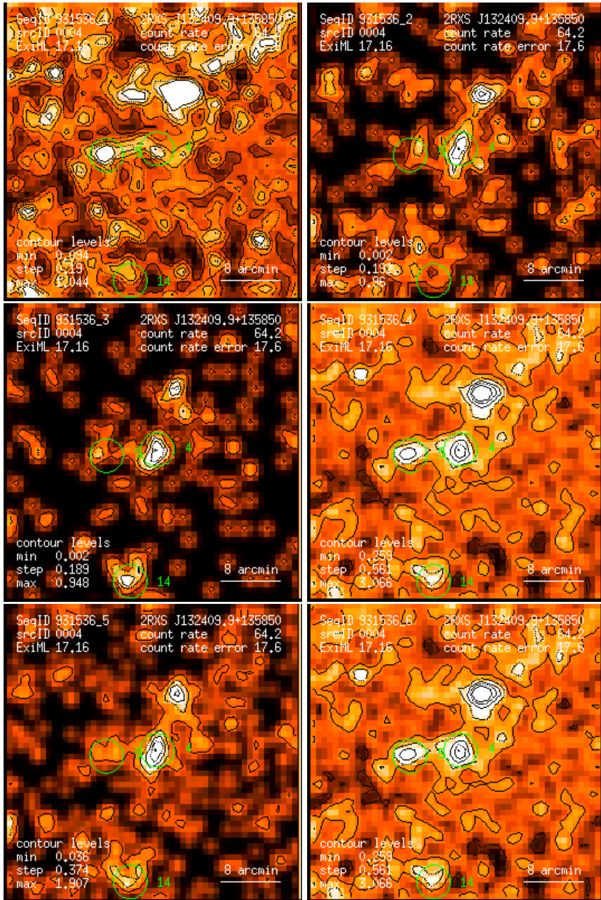
Figure 4: RASS 931536: detection 0004: band rate images, Gaussian filter: (1) PSPC channels 11 – 41, (2) 52 – 90, (3) 91 – 201, (4) 11 – 235, (5) 52 – 201, (6) 11 – 201. Broad band rates in counts/ks. Band rate contour levels in counts/ks/arcmin 2 .
