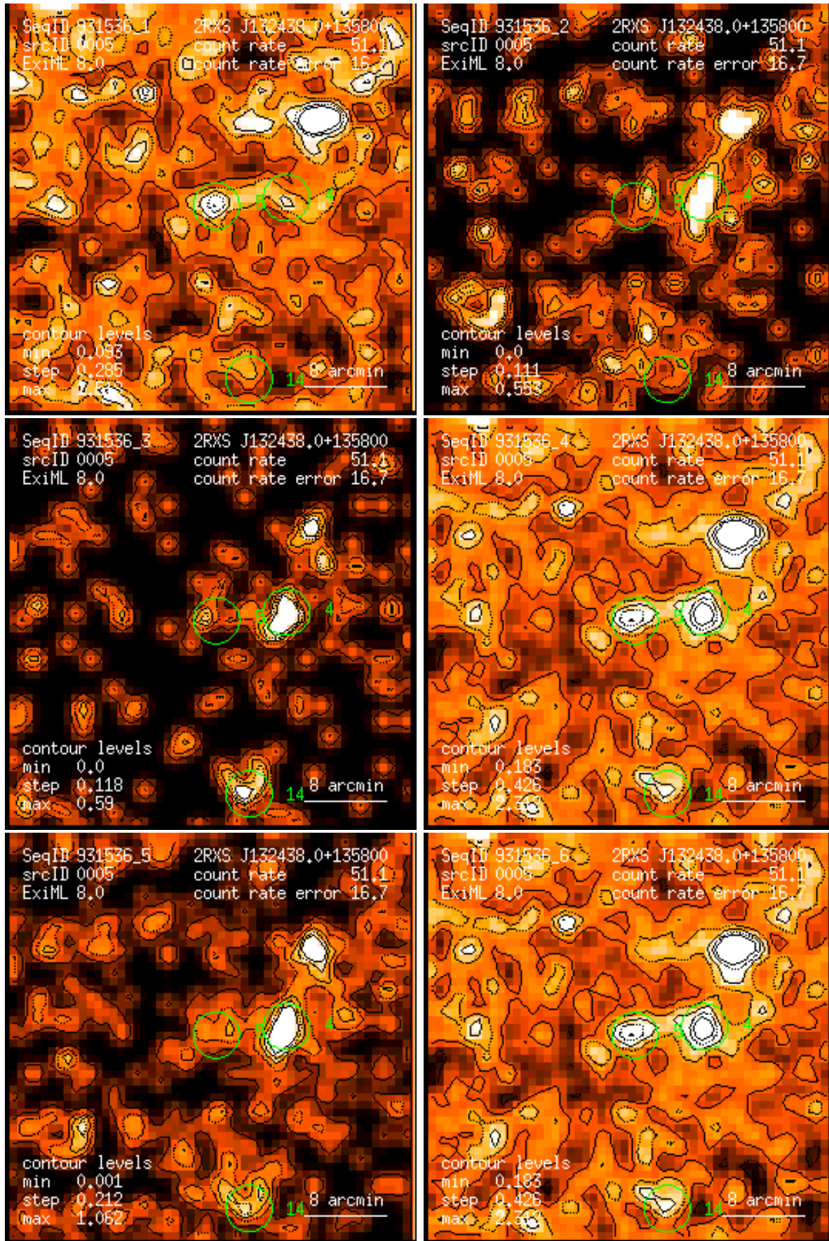
Figure 5: RASS 931536: detection 0005: band rate images, Gaussian filter: (1) PSPC channels 11 – 41, (2) 52 – 90, (3) 91 – 201, (4) 11 – 235, (5) 52 – 201, (6) 11 – 201. Broad band rates in counts/ks. Band rate contour levels in counts/ks/arcmin 2 .
