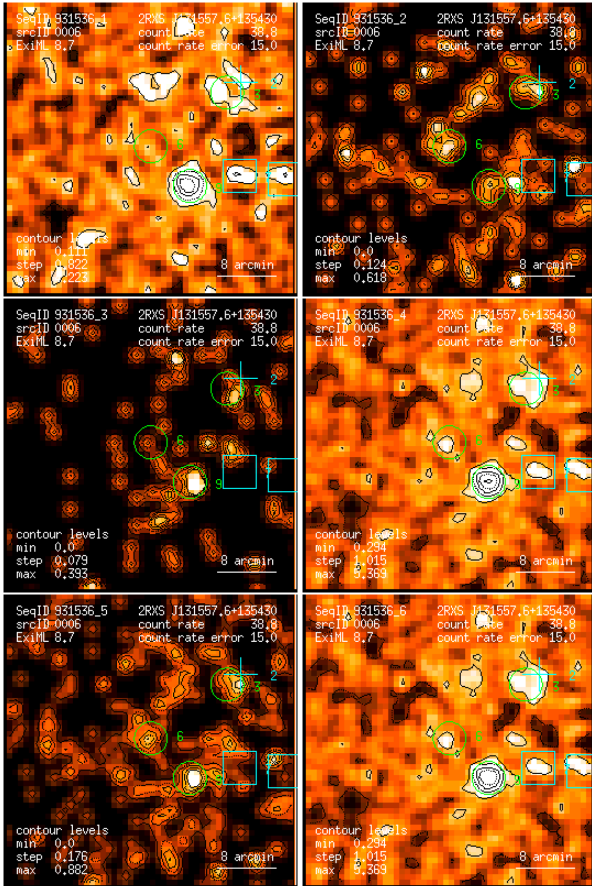
Figure 6: RASS 931536: detection 0006: band rate images, Gaussian filter: (1) PSPC channels 11 – 41, (2) 52 – 90, (3) 91 – 201, (4) 11 – 235, (5) 52 – 201, (6) 11 – 201. Broad band rates in counts/ks. Band rate contour levels in counts/ks/arcmin 2 .
