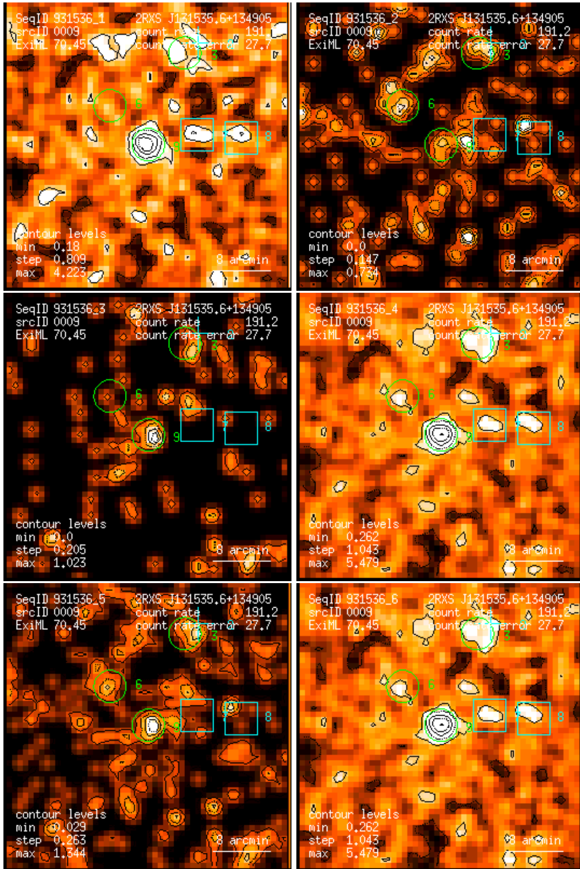
Figure 9: RASS 931536: detection 0009: band rate images, Gaussian filter: (1) PSPC channels 11 – 41, (2) 52 – 90, (3) 91 – 201, (4) 11 – 235, (5) 52 – 201, (6) 11 – 201. Broad band rates in counts/ks. Band rate contour levels in counts/ks/arcmin 2 .
