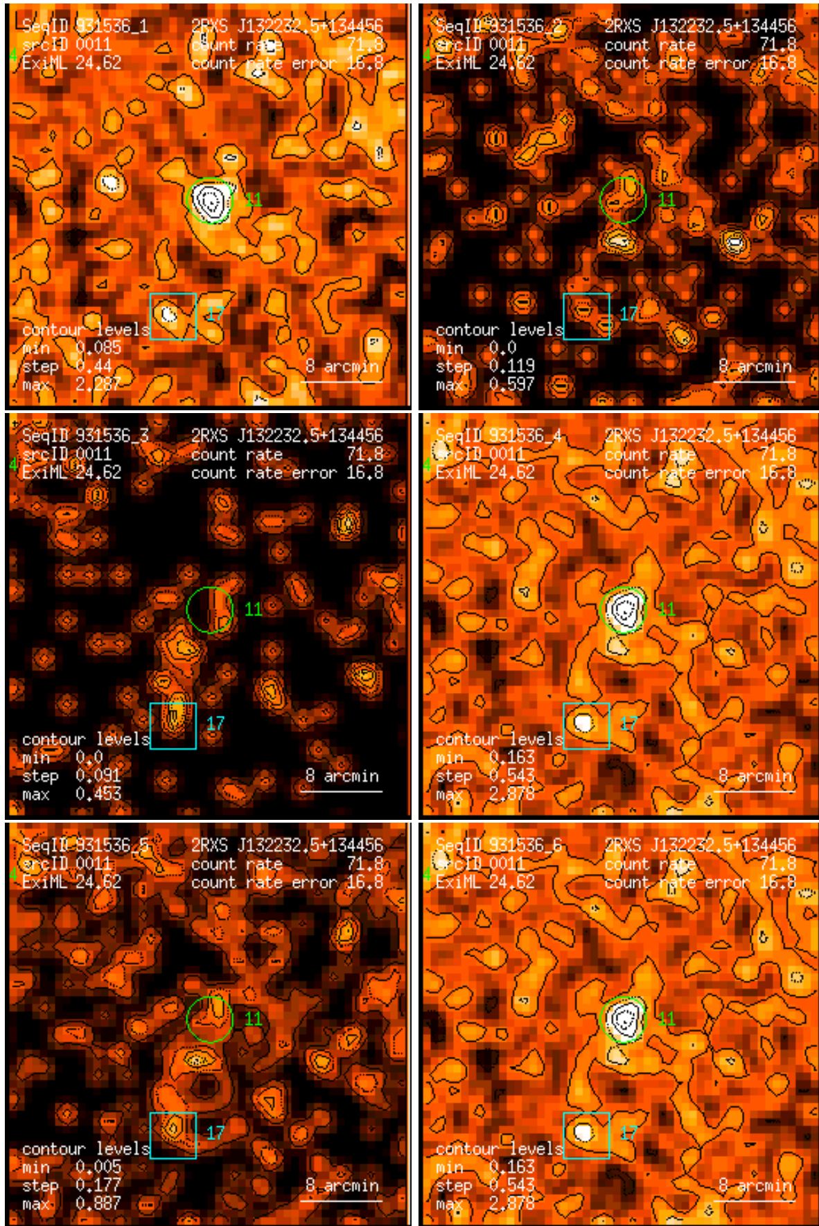
Figure 11: RASS 931536: detection 0011: band rate images, Gaussian filter: (1) PSPC channels 11 – 41, (2) 52 – 90, (3) 91 – 201, (4) 11 – 235, (5) 52 – 201, (6) 11 – 201. Broad band rates in counts/ks. Band rate contour levels in counts/ks/arcmin 2 .
