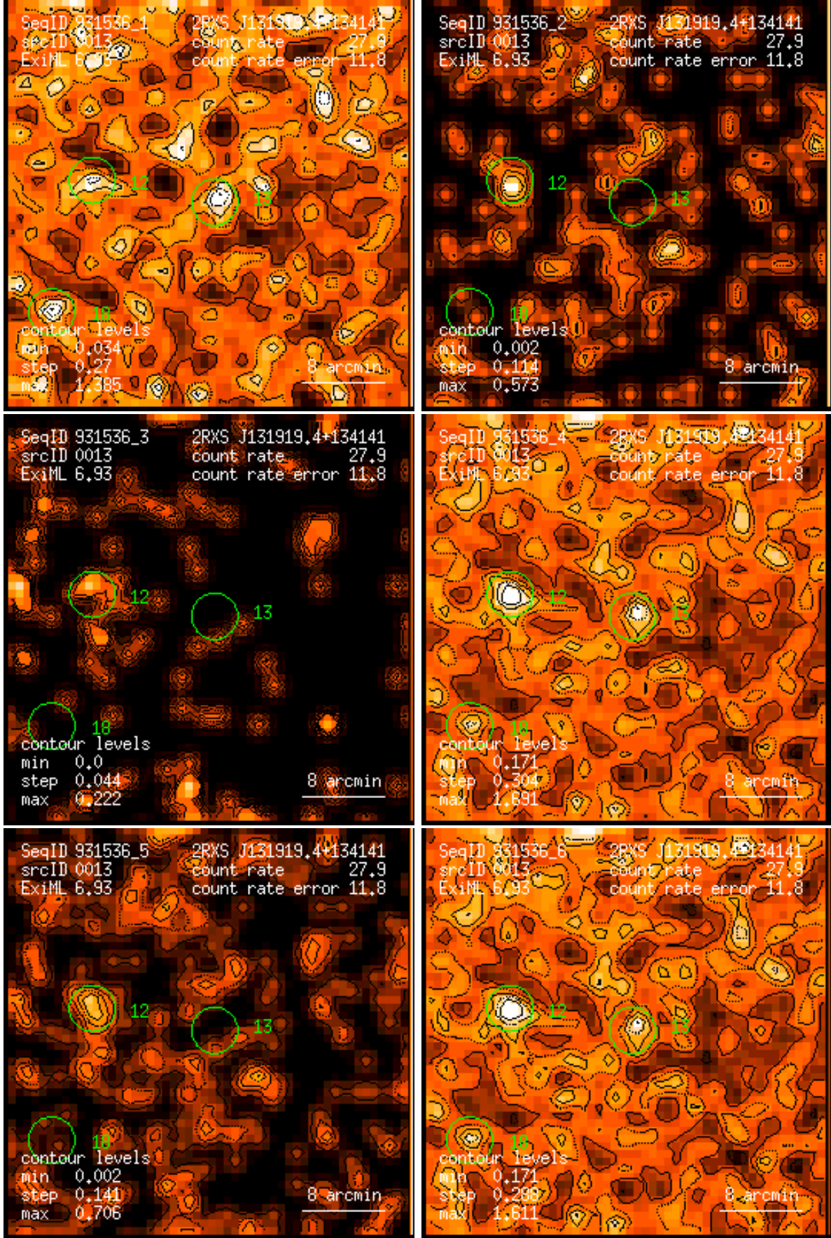
Figure 13: RASS 931536: detection 0013: band rate images, Gaussian filter: (1) PSPC channels 11 – 41, (2) 52 – 90, (3) 91 – 201, (4) 11 – 235, (5) 52 – 201, (6) 11 – 201. Broad band rates in counts/ks. Band rate contour levels in counts/ks/arcmin 2 .
