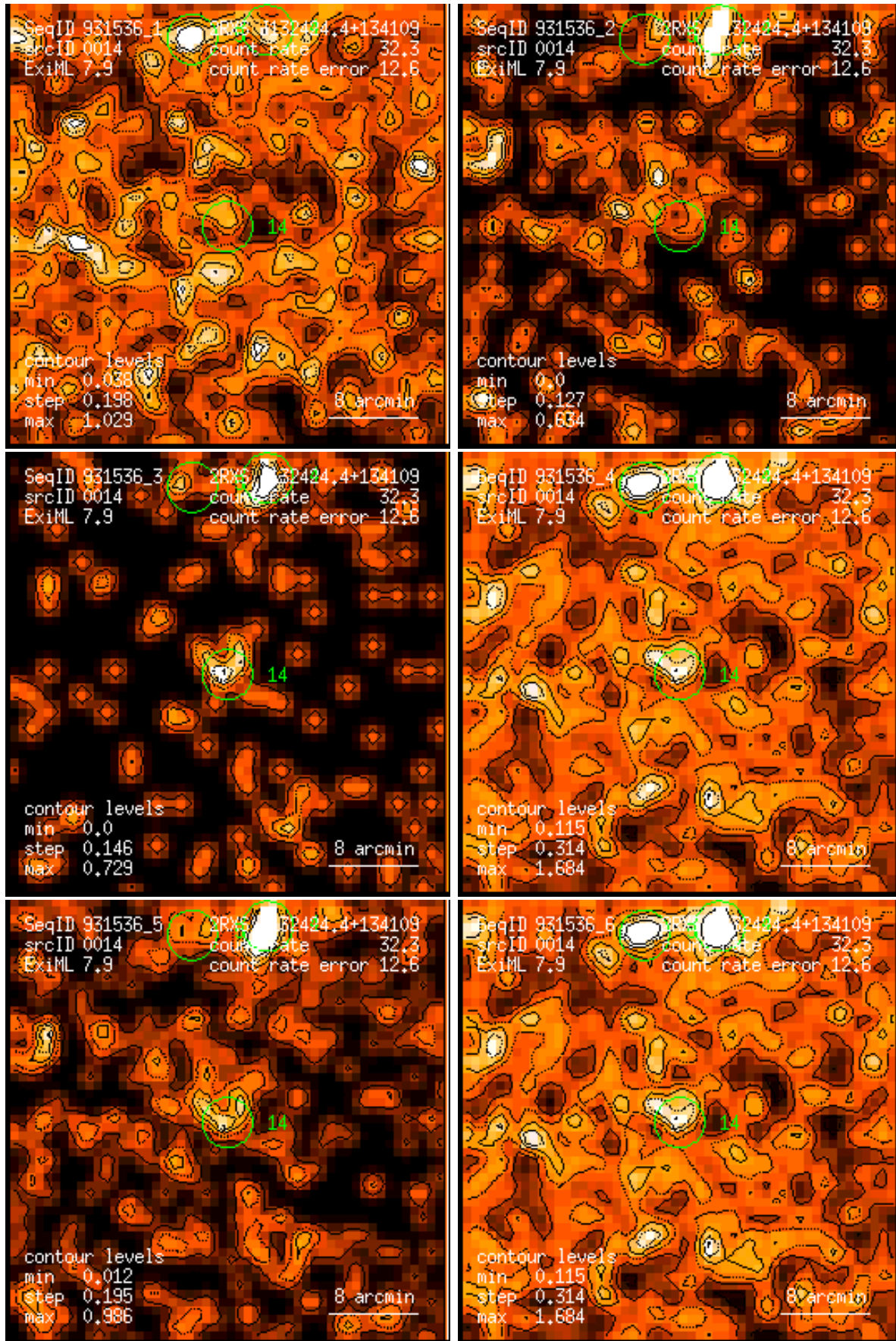
Figure 14: RASS 931536: detection 0014: band rate images, Gaussian filter: (1) PSPC channels 11 – 41, (2) 52 – 90, (3) 91 – 201, (4) 11 – 235, (5) 52 – 201, (6) 11 – 201. Broad band rates in counts/ks. Band rate contour levels in counts/ks/arcmin 2 .
