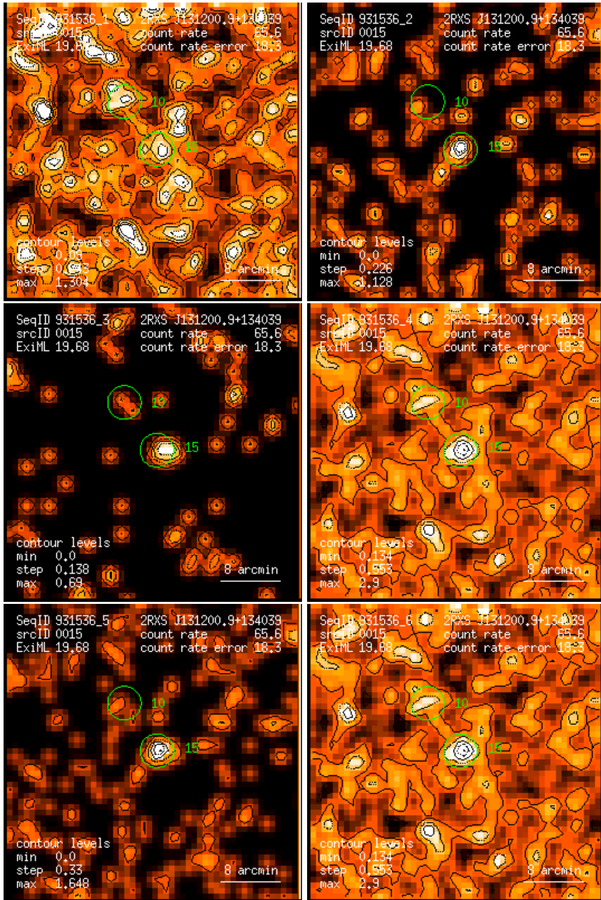
Figure 15: RASS 931536: detection 0015: band rate images, Gaussian filter: (1) PSPC channels 11 – 41, (2) 52 – 90, (3) 91 – 201, (4) 11 – 235, (5) 52 – 201, (6) 11 – 201. Broad band rates in counts/ks. Band rate contour levels in counts/ks/arcmin 2 .
