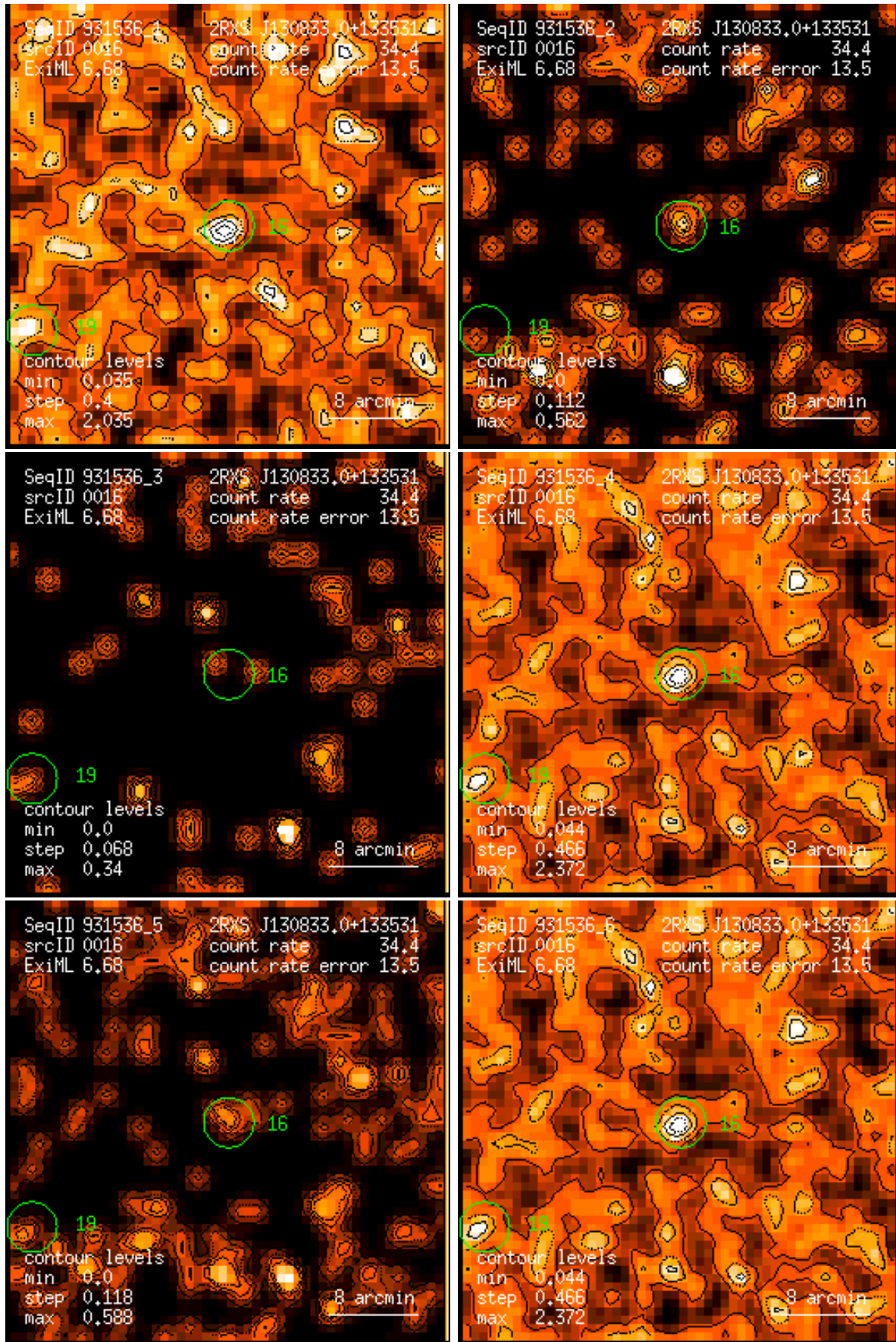
Figure 16: RASS 931536: detection 0016: band rate images, Gaussian filter: (1) PSPC channels 11 – 41, (2) 52 – 90, (3) 91 – 201, (4) 11 – 235, (5) 52 – 201, (6) 11 – 201. Broad band rates in counts/ks. Band rate contour levels in counts/ks/arcmin 2 .
