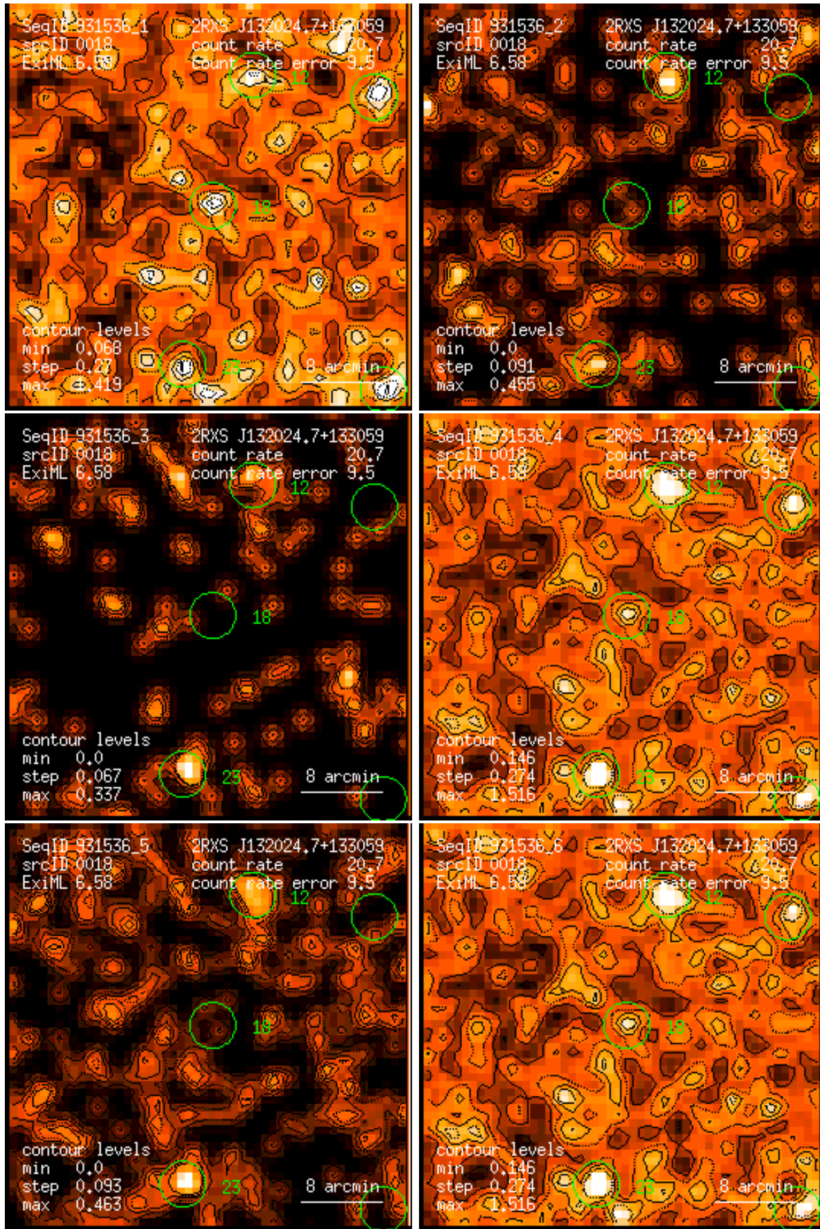
Figure 18: RASS 931536: detection 0018: band rate images, Gaussian filter: (1) PSPC channels 11 – 41, (2) 52 – 90, (3) 91 – 201, (4) 11 – 235, (5) 52 – 201, (6) 11 – 201. Broad band rates in counts/ks. Band rate contour levels in counts/ks/arcmin 2 .
