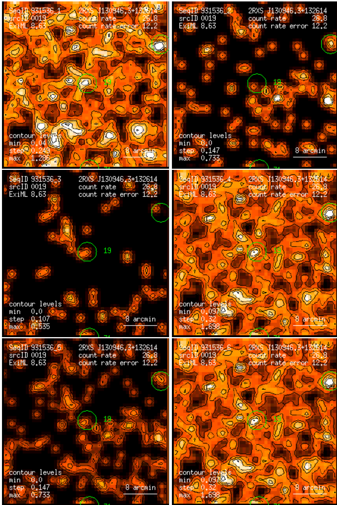
Figure 19: RASS 931536: detection 0019: band rate images, Gaussian filter: (1) PSPC channels 11 – 41, (2) 52 – 90, (3) 91 – 201, (4) 11 – 235, (5) 52 – 201, (6) 11 – 201. Broad band rates in counts/ks. Band rate contour levels in counts/ks/arcmin 2 .
