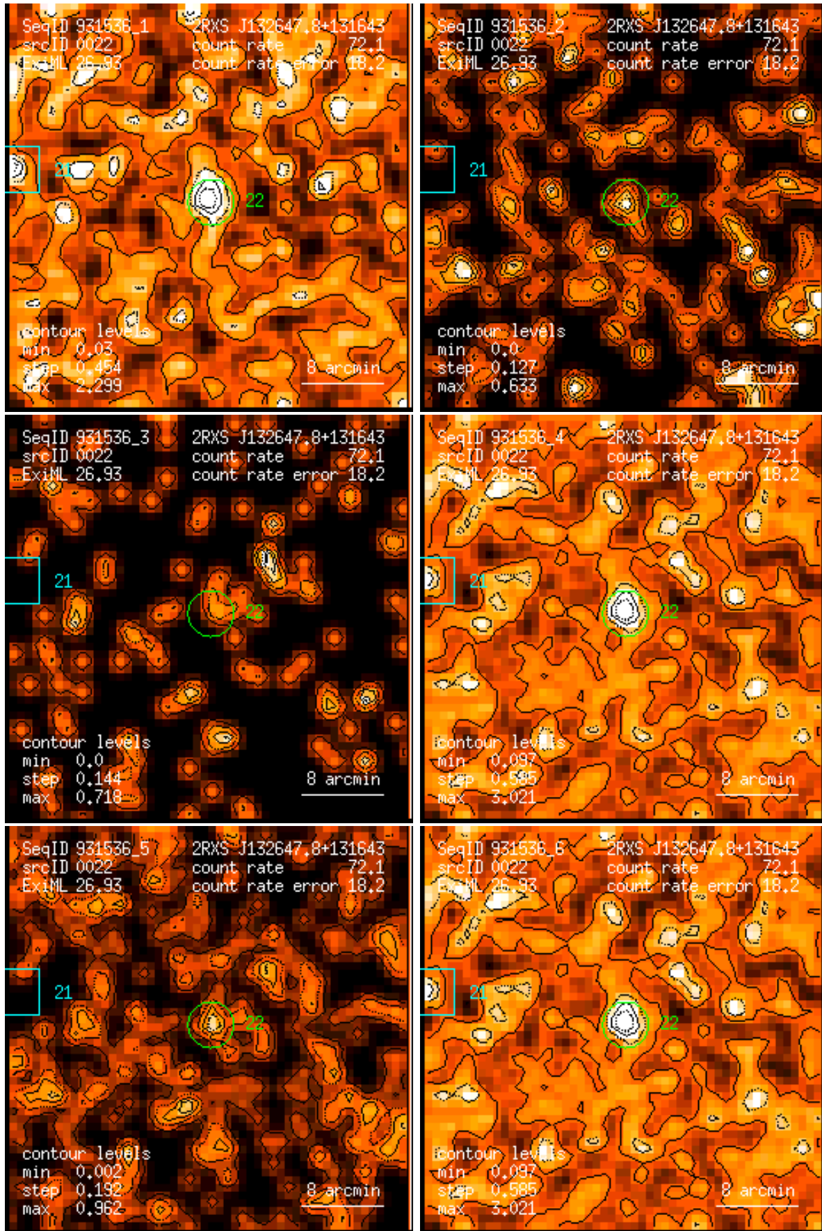
Figure 22: RASS 931536: detection 0022: band rate images, Gaussian filter: (1) PSPC channels 11 – 41, (2) 52 – 90, (3) 91 – 201, (4) 11 – 235, (5) 52 – 201, (6) 11 – 201. Broad band rates in counts/ks. Band rate contour levels in counts/ks/arcmin 2 .
