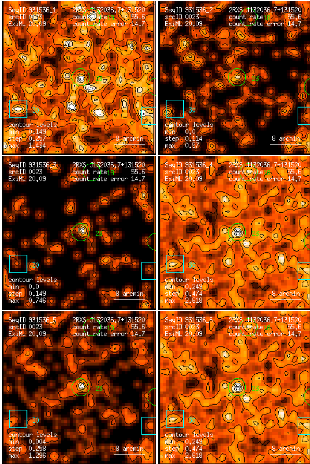
Figure 23: RASS 931536: detection 0023: band rate images, Gaussian filter: (1) PSPC channels 11 – 41, (2) 52 – 90, (3) 91 – 201, (4) 11 – 235, (5) 52 – 201, (6) 11 – 201. Broad band rates in counts/ks. Band rate contour levels in counts/ks/arcmin 2 .
