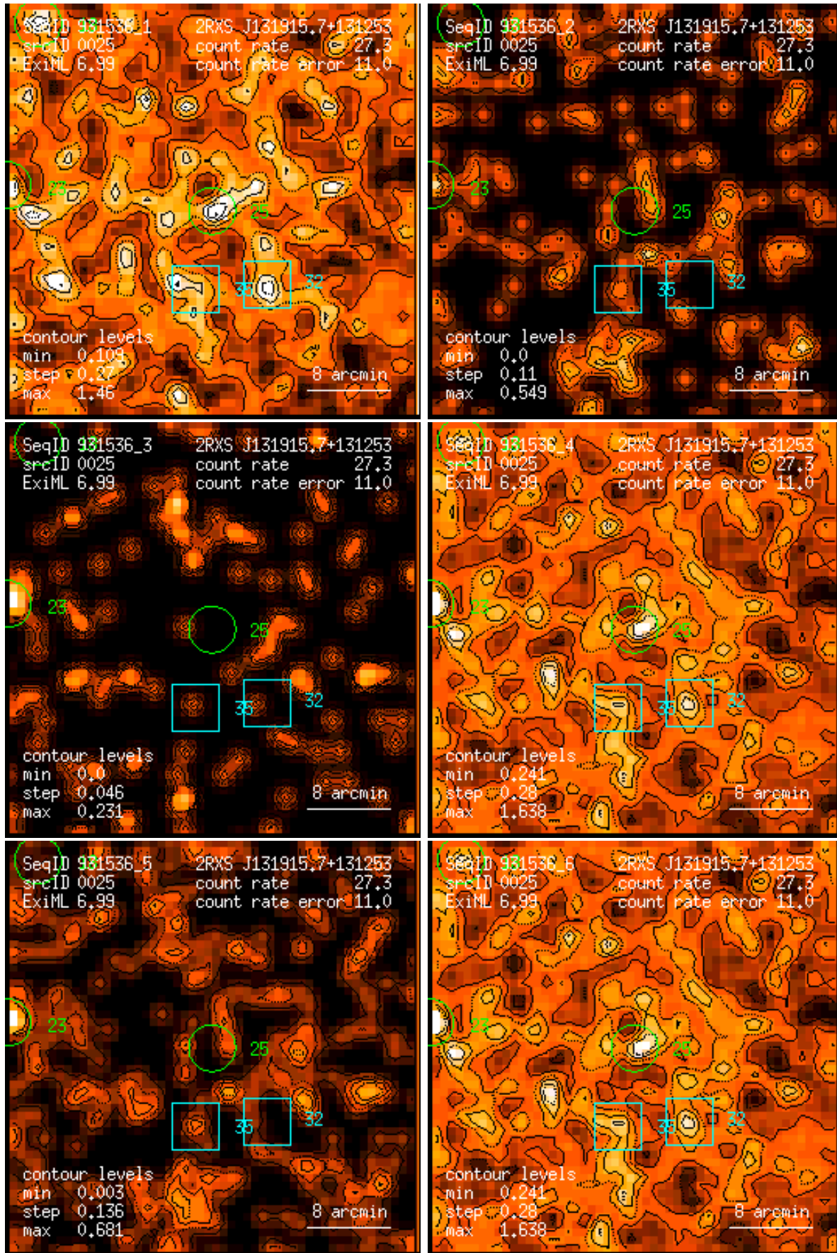
Figure 25: RASS 931536: detection 0025: band rate images, Gaussian filter: (1) PSPC channels 11 – 41, (2) 52 – 90, (3) 91 – 201, (4) 11 – 235, (5) 52 – 201, (6) 11 – 201. Broad band rates in counts/ks. Band rate contour levels in counts/ks/arcmin 2 .
