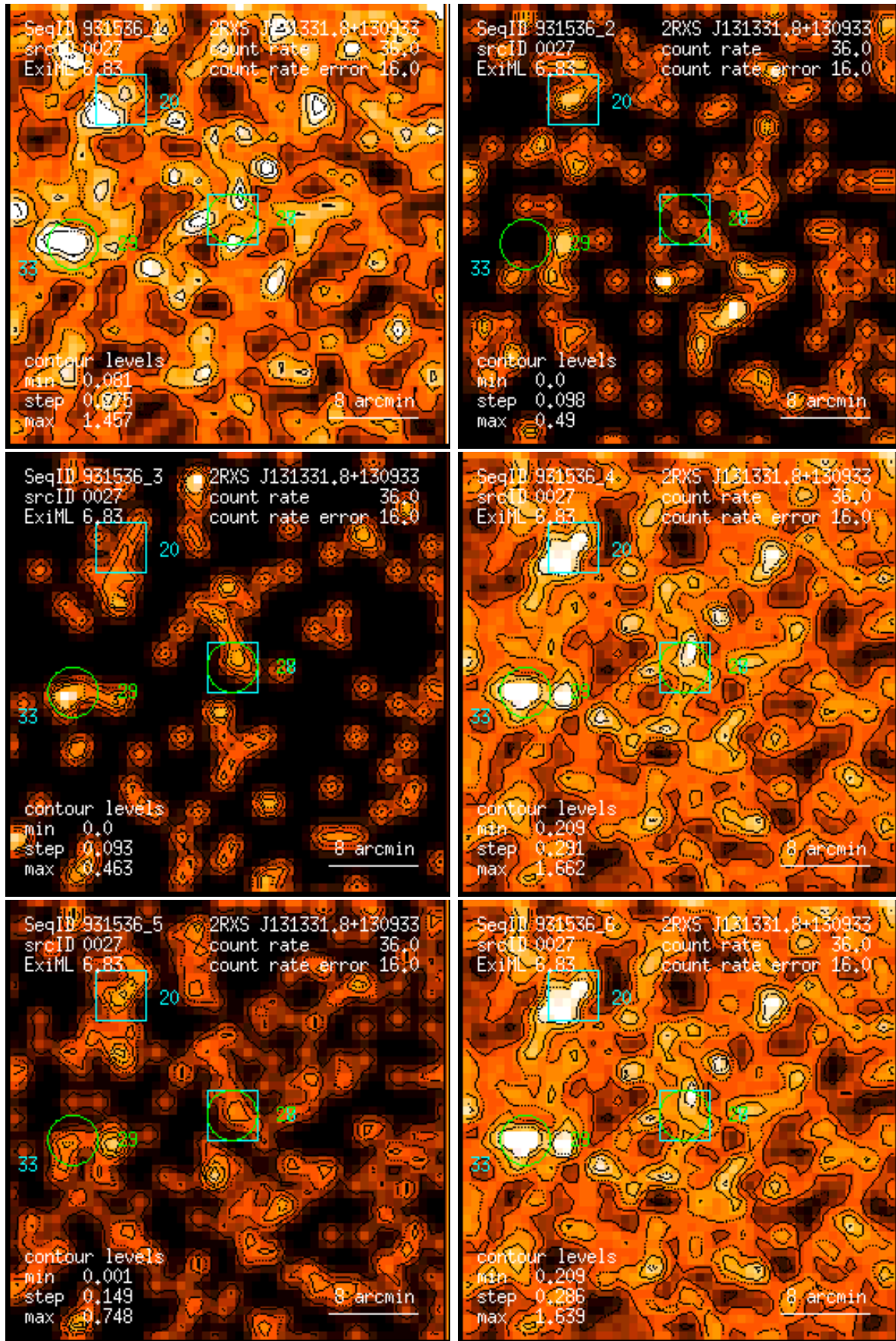
Figure 27: RASS 931536: detection 0027: band rate images, Gaussian filter: (1) PSPC channels 11 – 41, (2) 52 – 90, (3) 91 – 201, (4) 11 – 235, (5) 52 – 201, (6) 11 – 201. Broad band rates in counts/ks. Band rate contour levels in counts/ks/arcmin 2 .
