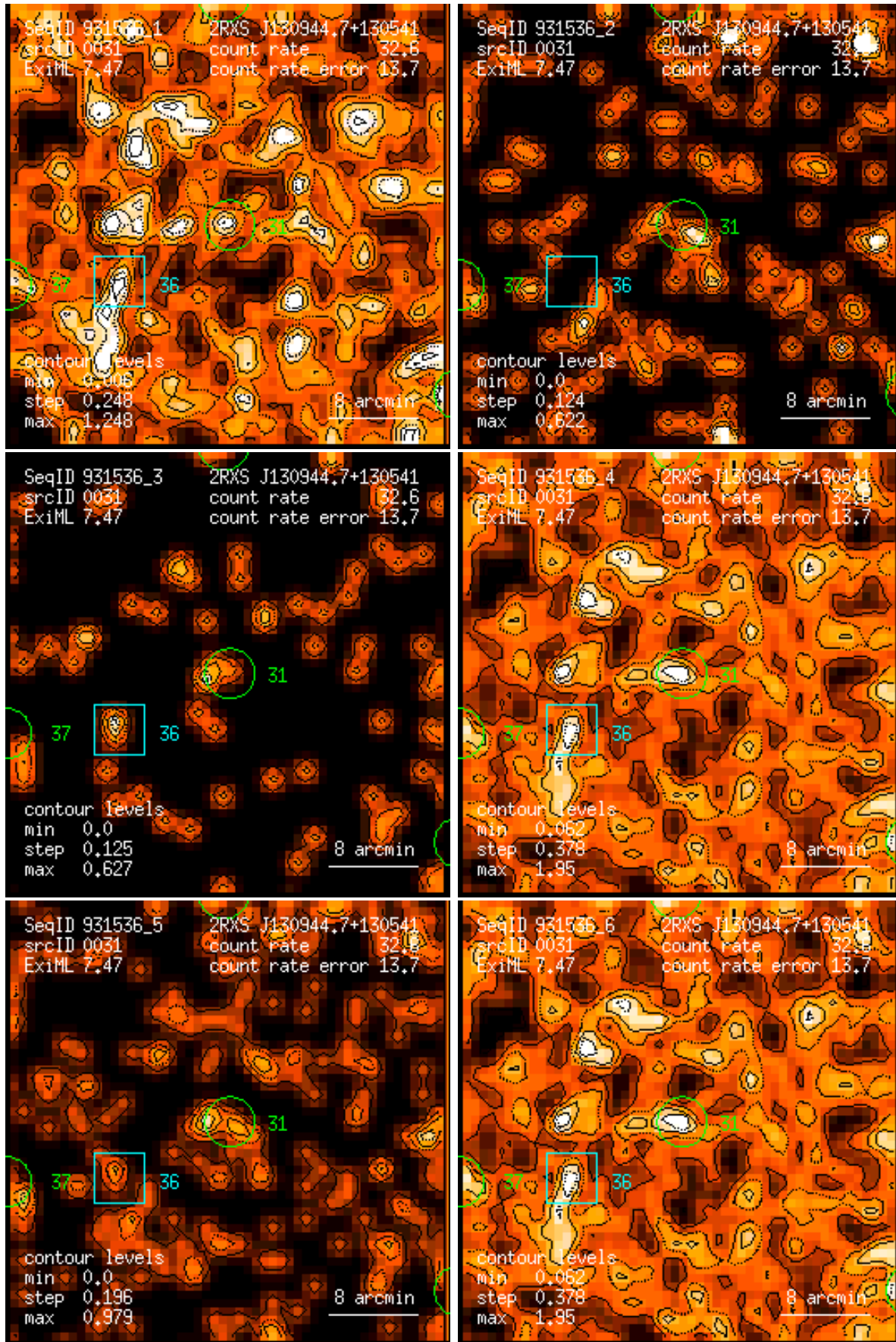
Figure 31: RASS 931536: detection 0031: band rate images, Gaussian filter: (1) PSPC channels 11 – 41, (2) 52 – 90, (3) 91 – 201, (4) 11 – 235, (5) 52 – 201, (6) 11 – 201. Broad band rates in counts/ks. Band rate contour levels in counts/ks/arcmin 2 .
