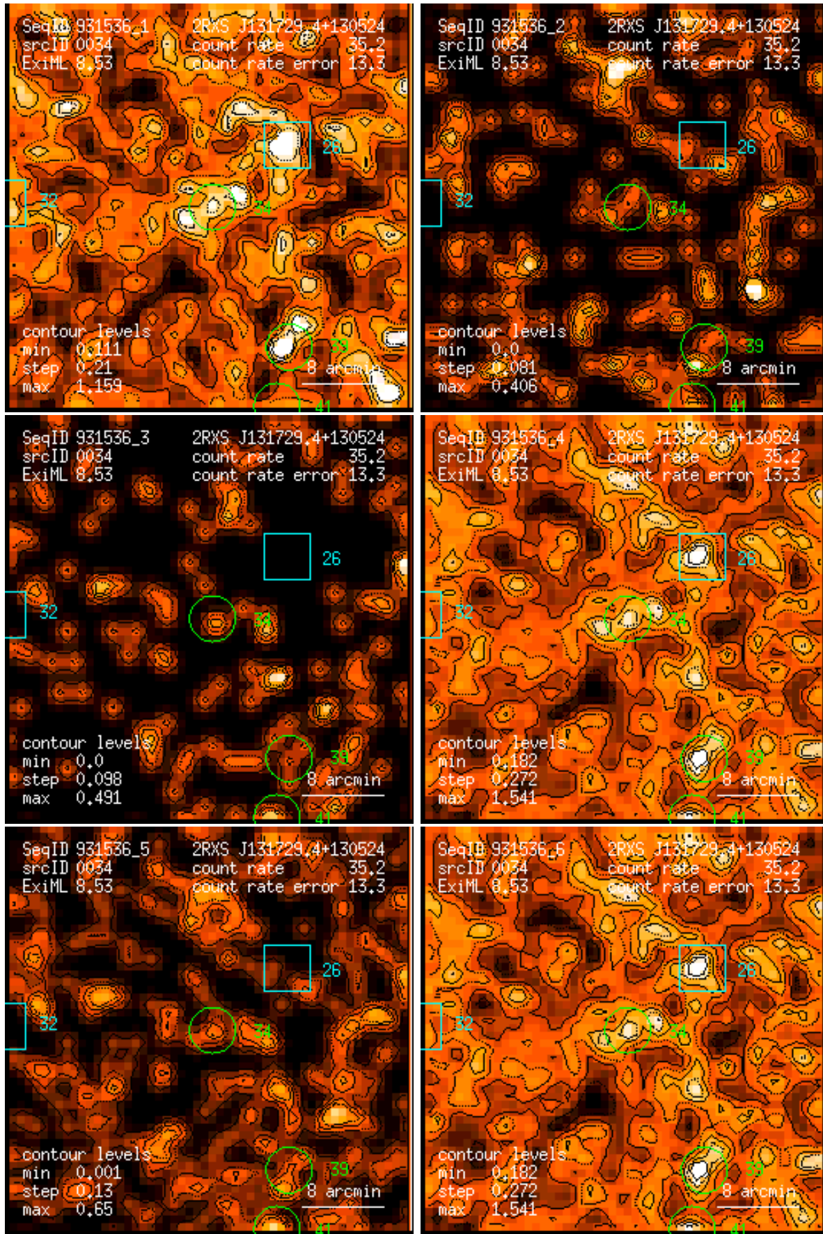
Figure 34: RASS 931536: detection 0034: band rate images, Gaussian filter: (1) PSPC channels 11 – 41, (2) 52 – 90, (3) 91 – 201, (4) 11 – 235, (5) 52 – 201, (6) 11 – 201. Broad band rates in counts/ks. Band rate contour levels in counts/ks/arcmin 2 .
