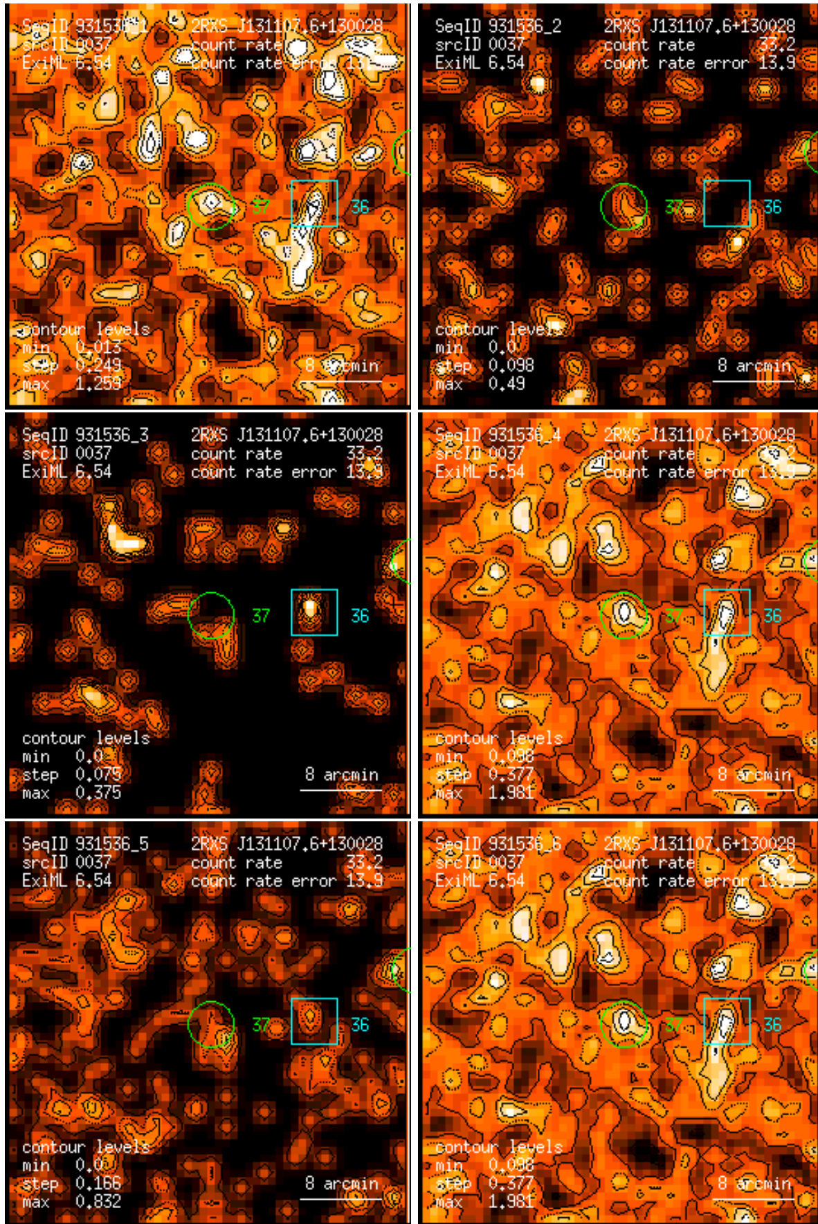
Figure 37: RASS 931536: detection 0037: band rate images, Gaussian filter: (1) PSPC channels 11 – 41, (2) 52 – 90, (3) 91 – 201, (4) 11 – 235, (5) 52 – 201, (6) 11 – 201. Broad band rates in counts/ks. Band rate contour levels in counts/ks/arcmin 2 .
