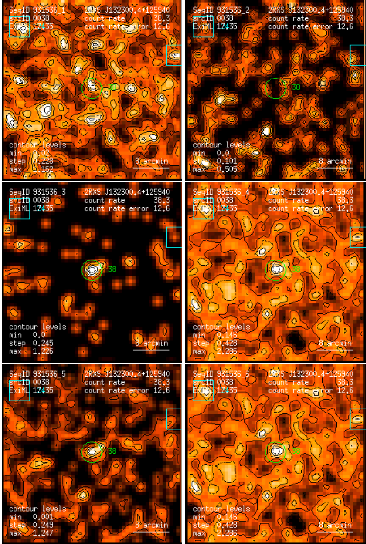
Figure 38: RASS 931536: detection 0038: band rate images, Gaussian filter: (1) PSPC channels 11 – 41, (2) 52 – 90, (3) 91 – 201, (4) 11 – 235, (5) 52 – 201, (6) 11 – 201. Broad band rates in counts/ks. Band rate contour levels in counts/ks/arcmin 2 .
