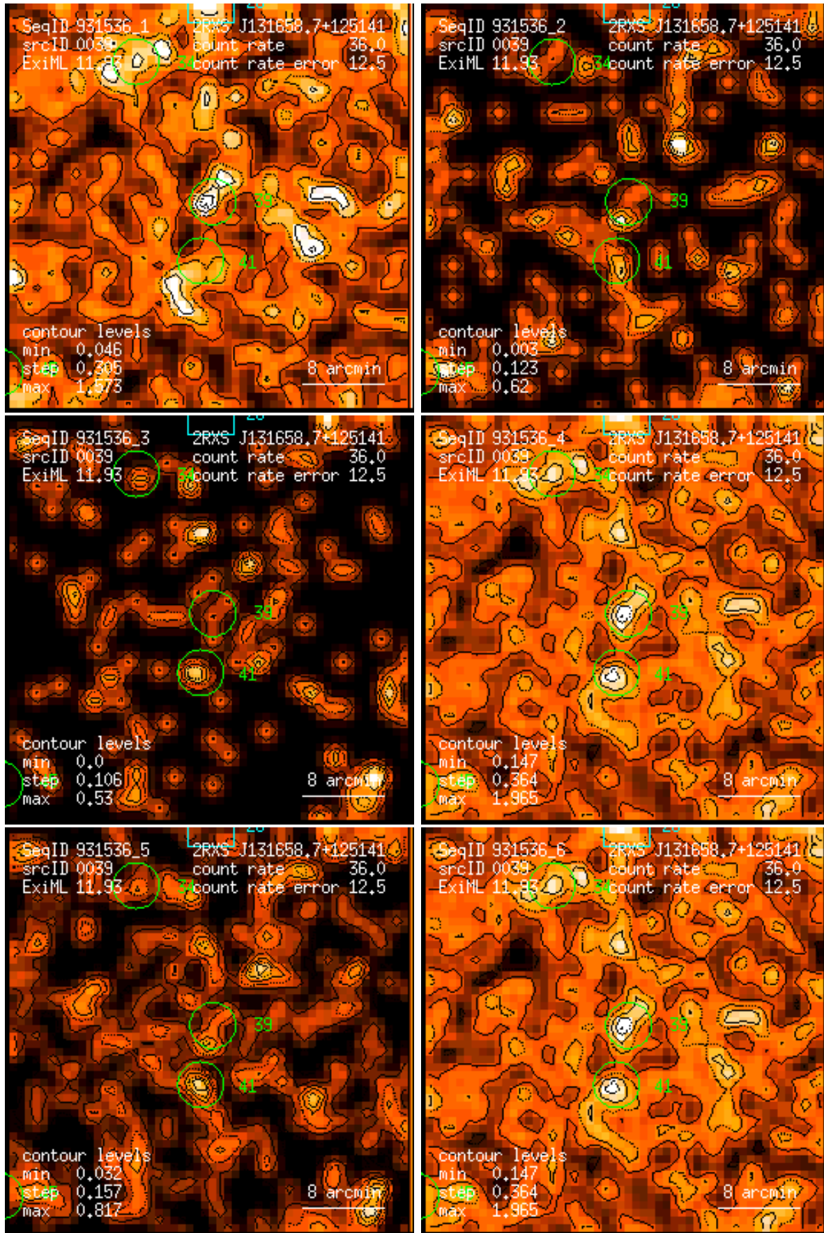
Figure 39: RASS 931536: detection 0039: band rate images, Gaussian filter: (1) PSPC channels 11 – 41, (2) 52 – 90, (3) 91 – 201, (4) 11 – 235, (5) 52 – 201, (6) 11 – 201. Broad band rates in counts/ks. Band rate contour levels in counts/ks/arcmin 2 .
