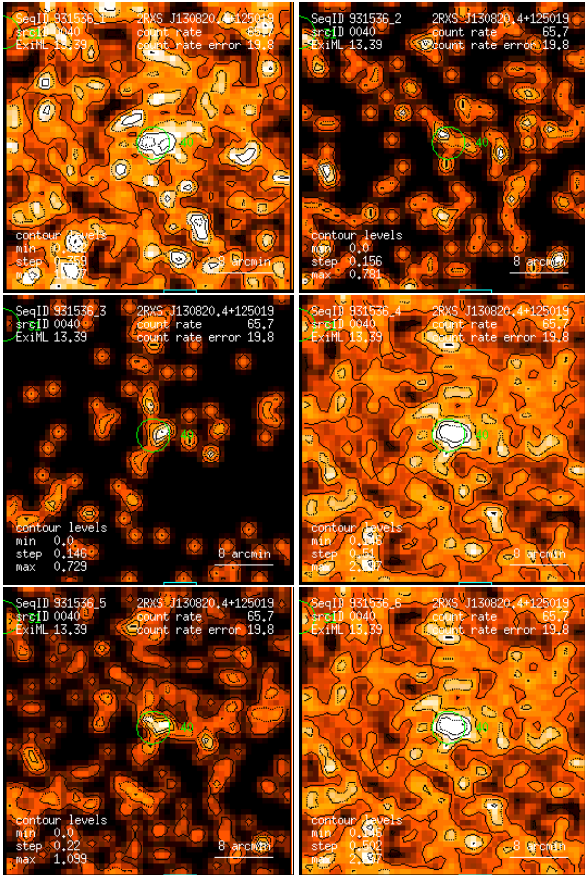
Figure 40: RASS 931536: detection 0040: band rate images, Gaussian filter: (1) PSPC channels 11 – 41, (2) 52 – 90, (3) 91 – 201, (4) 11 – 235, (5) 52 – 201, (6) 11 – 201. Broad band rates in counts/ks. Band rate contour levels in counts/ks/arcmin 2 .
