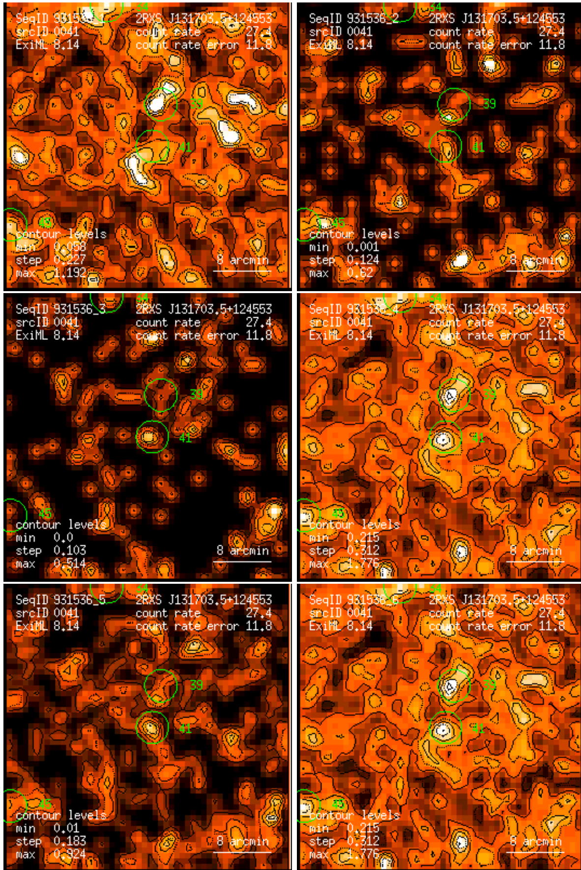
Figure 41: RASS 931536: detection 0041: band rate images, Gaussian filter: (1) PSPC channels 11 – 41, (2) 52 – 90, (3) 91 – 201, (4) 11 – 235, (5) 52 – 201, (6) 11 – 201. Broad band rates in counts/ks. Band rate contour levels in counts/ks/arcmin 2 .
