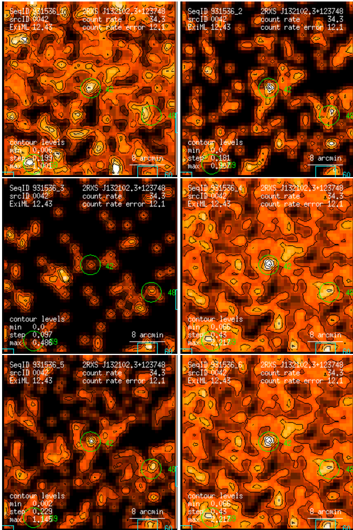
Figure 42: RASS 931536: detection 0042: band rate images, Gaussian filter: (1) PSPC channels 11 – 41, (2) 52 – 90, (3) 91 – 201, (4) 11 – 235, (5) 52 – 201, (6) 11 – 201. Broad band rates in counts/ks. Band rate contour levels in counts/ks/arcmin 2 .
